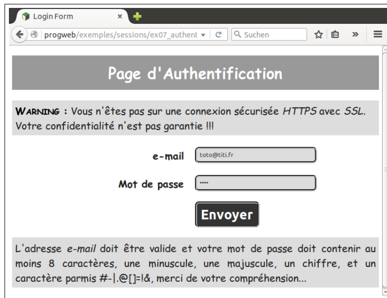
FIGURE 7.4 : Illustration du code source 7.9
