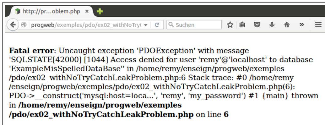
FIGURE 8.8 : Illustration du code source 8.4
