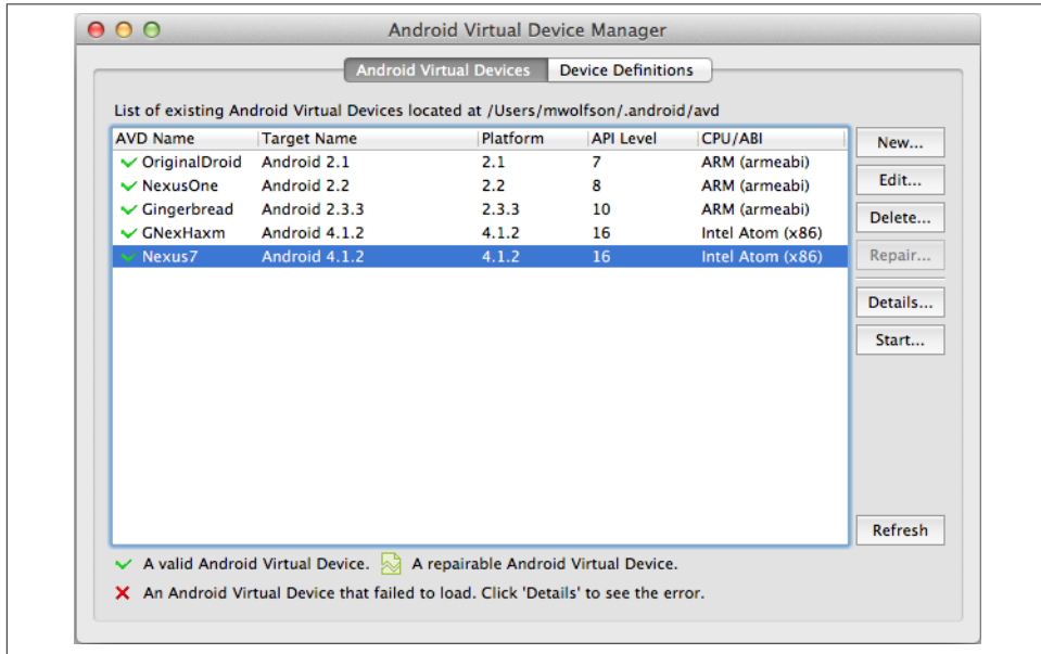
Figure 3-2. AVD Manager
