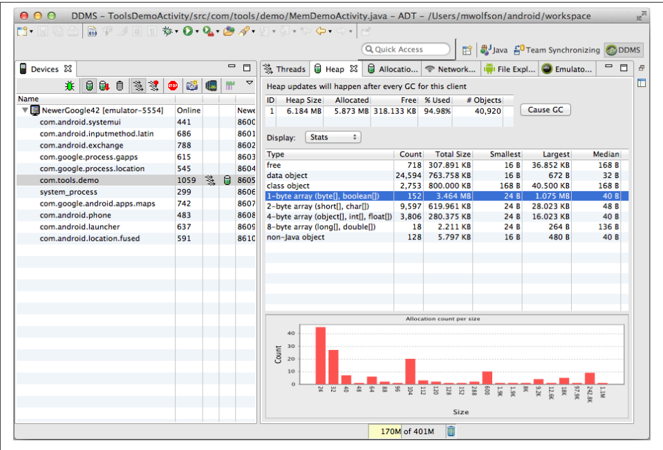
Figure 10-4. Heap view
