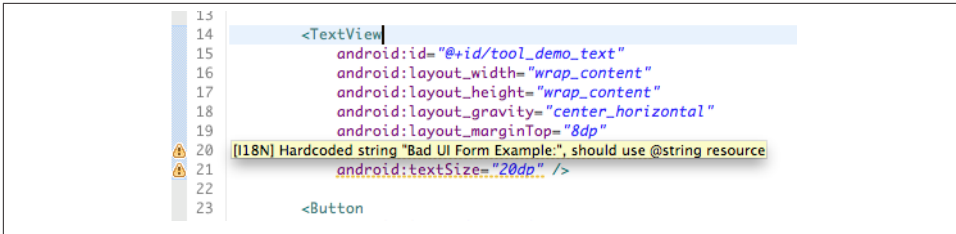
Figure 7-15. Lint warnings in XML file
