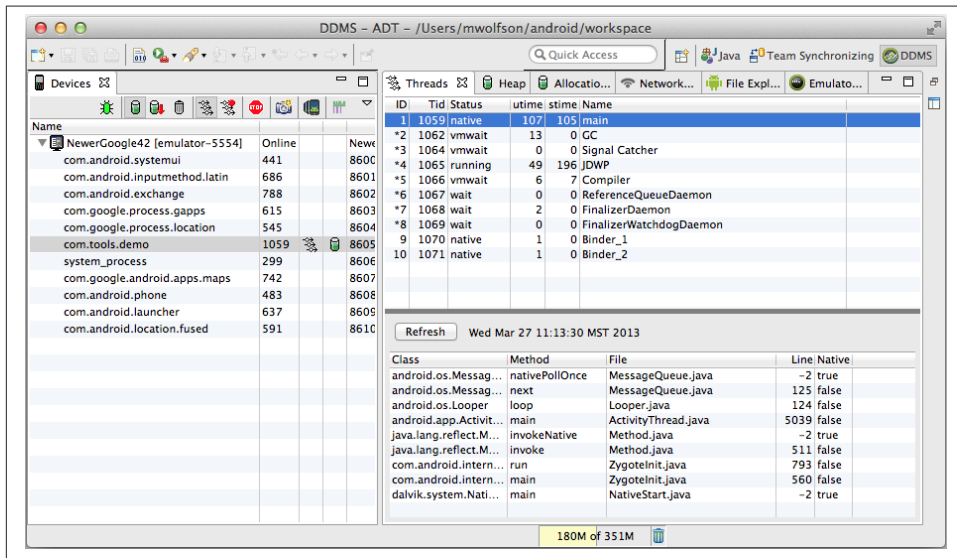
Figure 10-3. Viewing information about Heap execution
