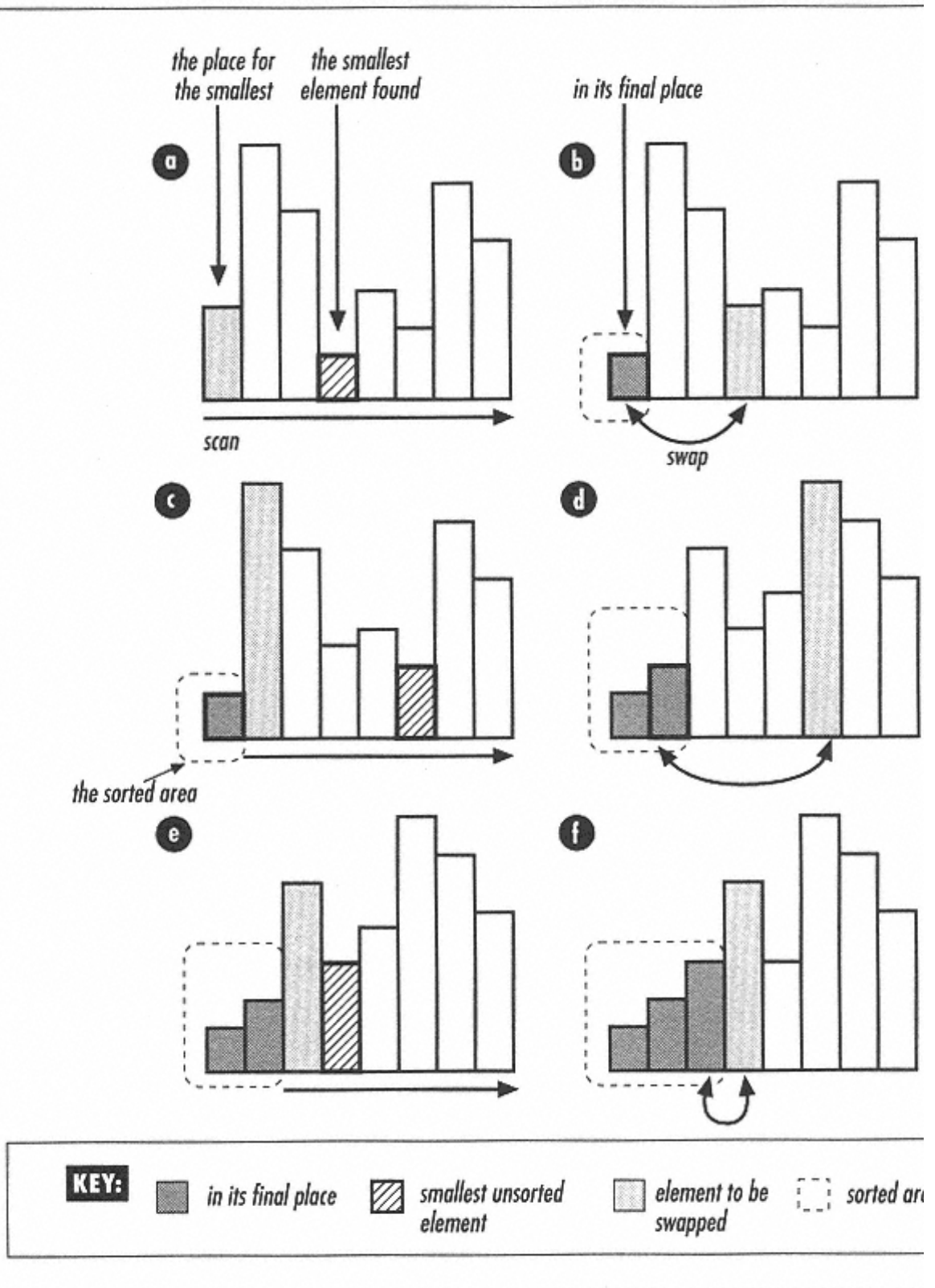
Figure 4-3. The first steps of selection sort: alternating minimum-finding scans and swaps
