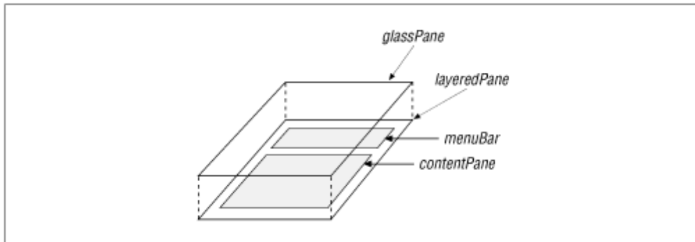
Figure 8.3. JRootPane
