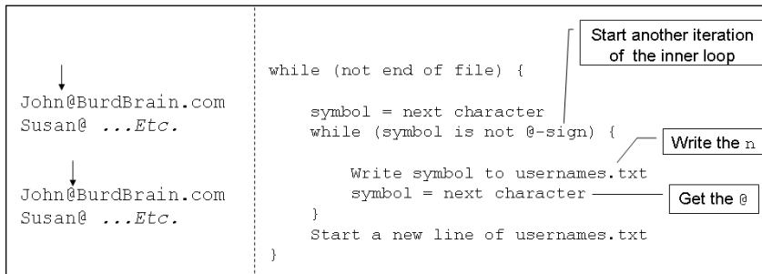
Figure 14-5: Reaching the end of the username.
