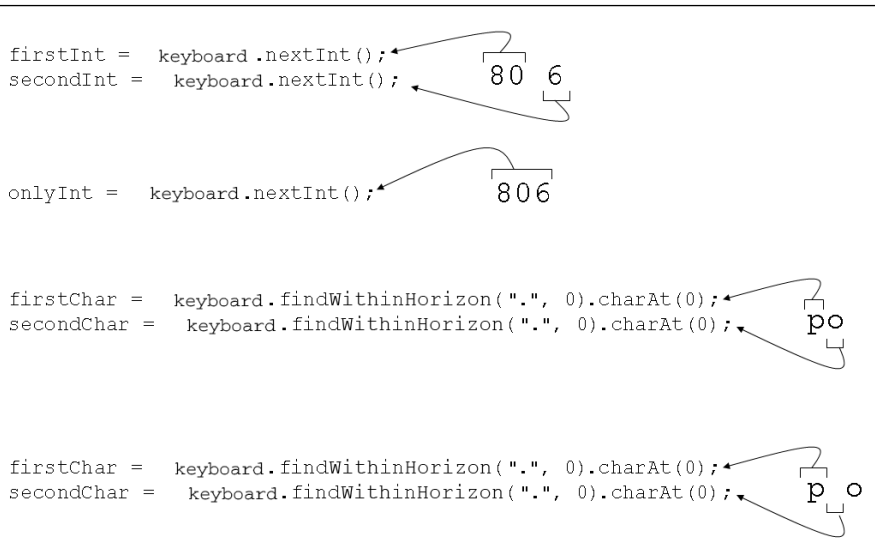
Figure 8-8: Reading num- bers and characters.
