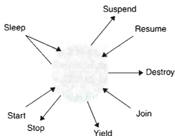
Figure 1-6 The control methods that affect a thread's behavior.
