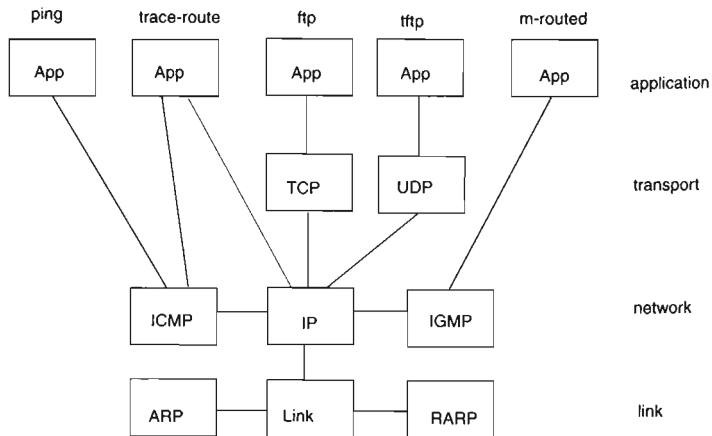
Figure 2-3 The TCP/IP suite.
