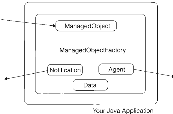
Figure 11-2 Modular design of JMAPI applications.
