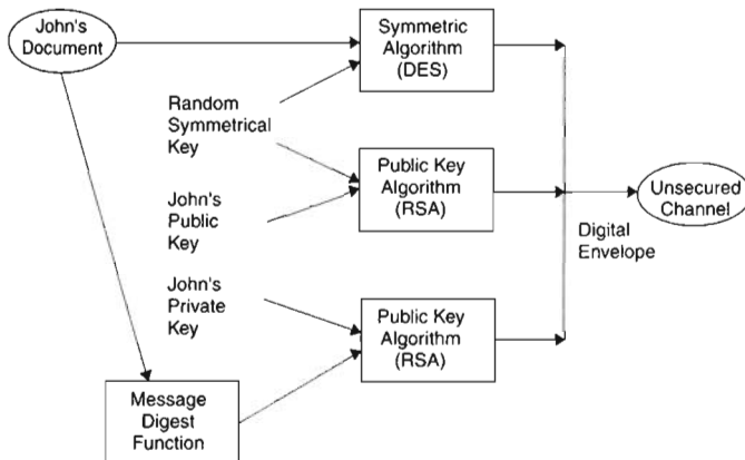
Figure 13-6 A combination of symmetric and asymmetric encryption.
