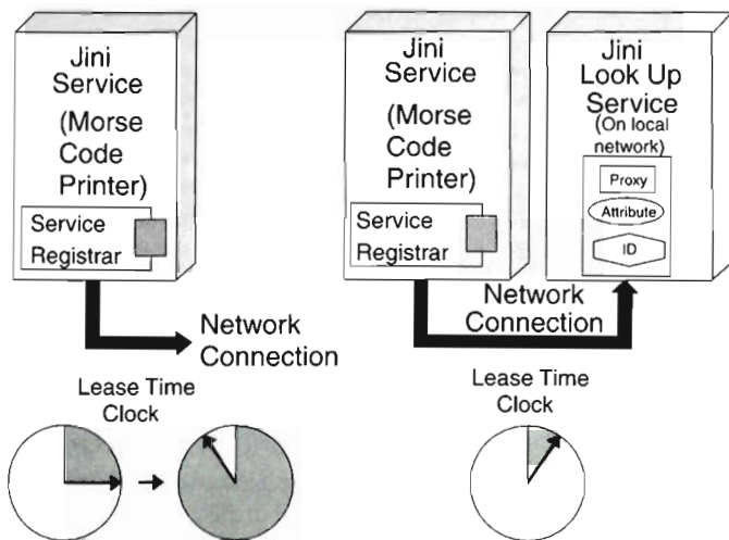
Figure 10-4 Jini Lease Renewal.
