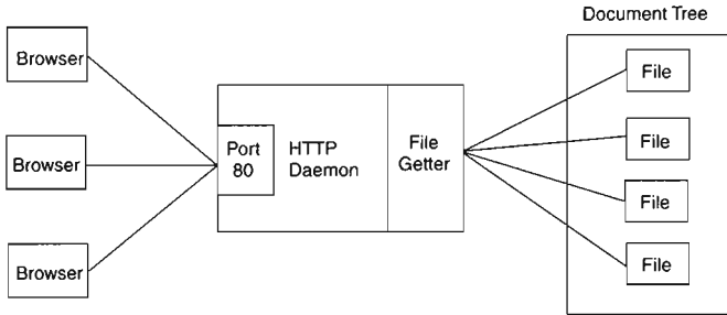
Figure 7-1 Web servers handle requests for multiple files.
