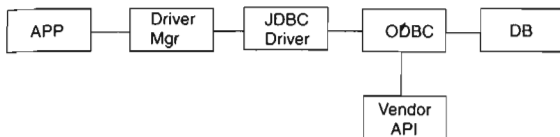
Figure 4-2 Type 1 JDBC/ODBC bridge.
