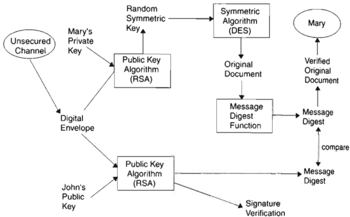
Figure 13-7 Decryption of example.
