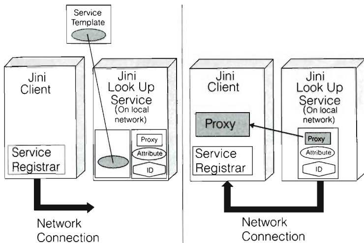
Figure 10-5 The Jini Client constructs a template identifying the desired service, and the JLUS matches this template against all registered service items and returns the proxy object from the matching service item.
