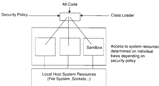
Figure 13-3 JDK 1.2 security model.
