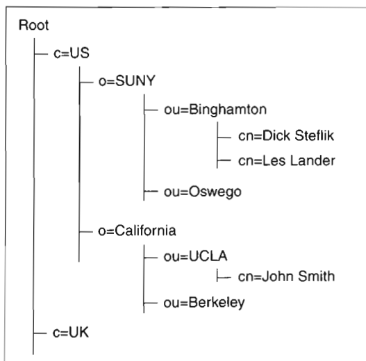
Figure 12-1 Distinguished name structure by geographic location.
