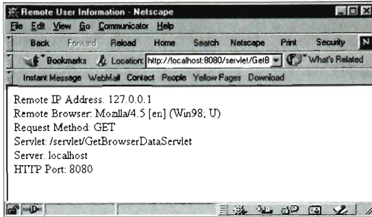
Figure 7-5 GetBrowserDataServlet output.
