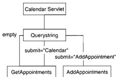
Figure 7-10 Calendar Servlet.
