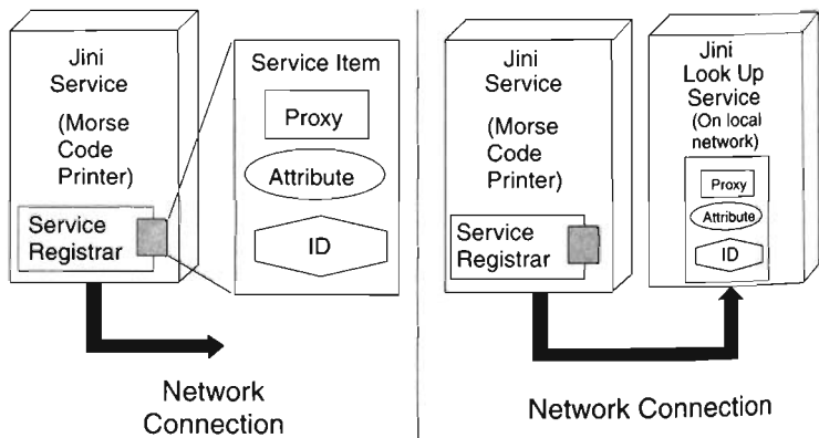
Figure 10-3 Jini Join.
