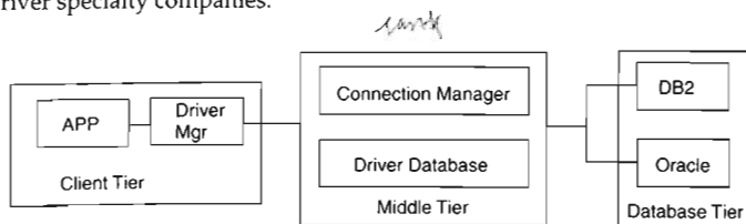
Figure 4-4 Type 3 driver.
