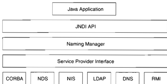
Figure 12-3 JNDI architecture.
