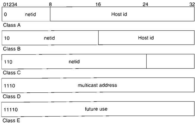
Figure 2-5 IP address classes.
