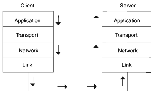
Figure 2-2 Data movement from one host to another.
