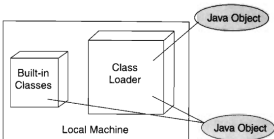
Figure 13-4 Downloaded Java objects use the local built-in classes rather than their own.
