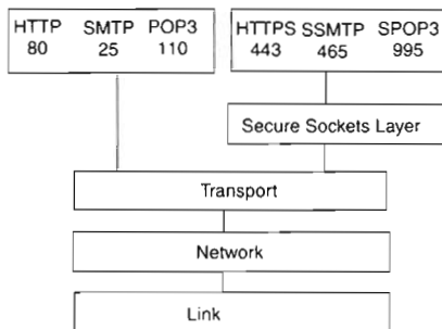
Figure 13-9 Secure Sockets Layer.
