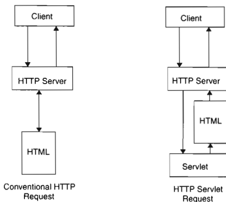
Figure 7-3 Servlets create documents on the fly rather than getting documents that were already there.
