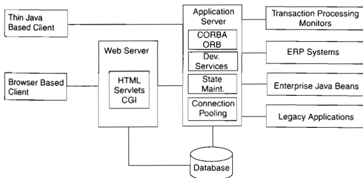
Figure 9-1 General application server architecture.
