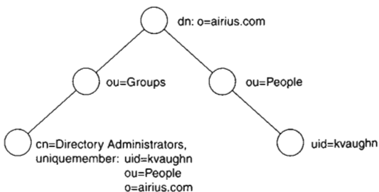
Figure 12-5 Airius.com.
