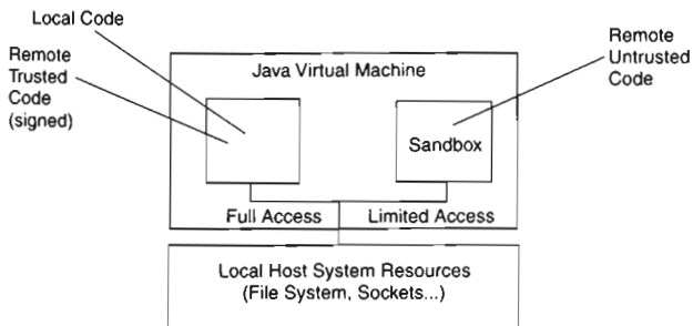
Figure 13-2 JDK 1.1 security model.
