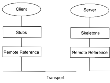
Figure 5-2 Java RMI architecture.
