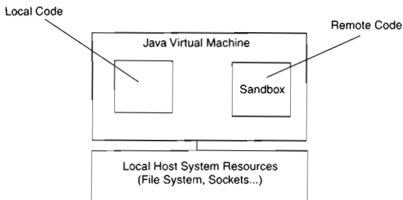
Figure 13-1 JDK 1.0 sandbox model.
