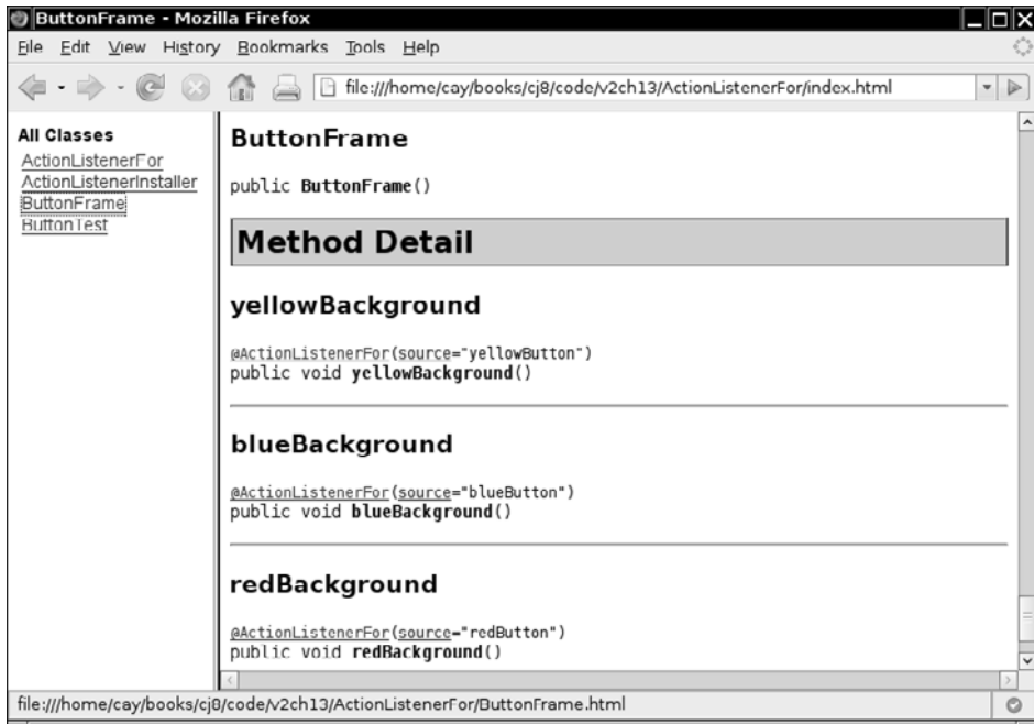
Figure 10.2 Documented annotations
