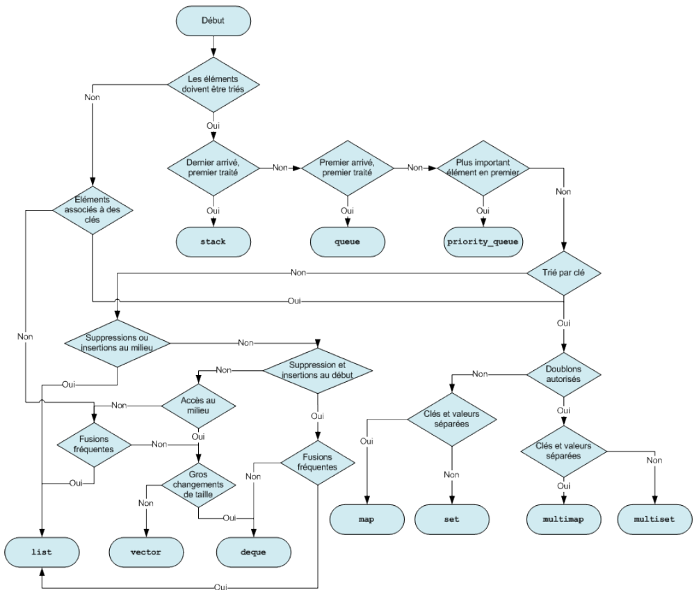
FIGURE 34.4 – Choisir le bon conteneur
