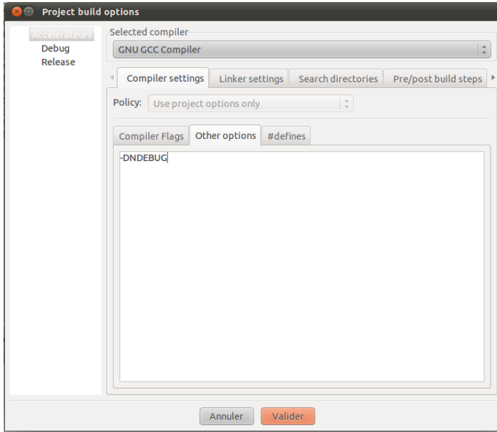
FIGURE 39.1 – Désactiver les assertions
