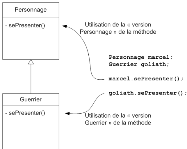
FIGURE 18.6 – Principe du masquage
