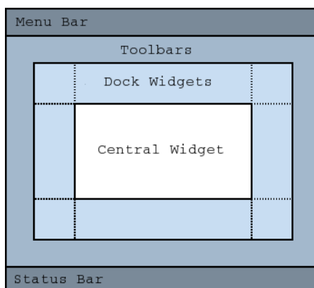
FIGURE 30.1 – Layout de la QMainWindow
