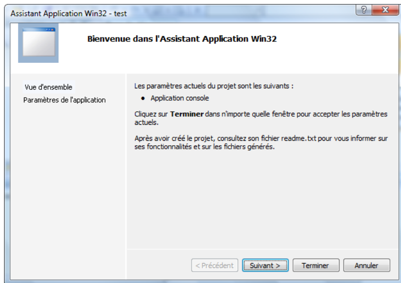
FIGURE 2.10 – Assistant application
