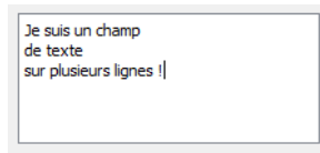
FIGURE 28.16 – QTextEdit
