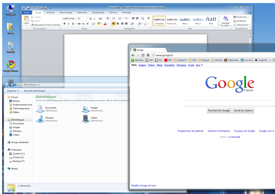
FIGURE 1.1 – Des programmes
