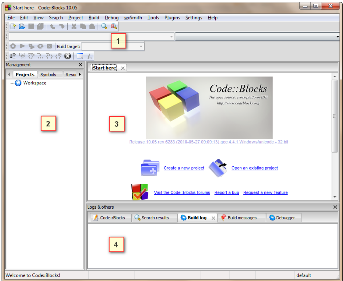
FIGURE 2.2 – Code Blocks
