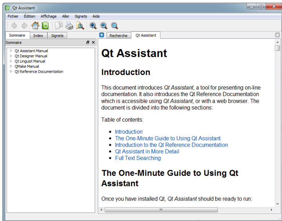
FIGURE 26.3 – Qt Assistant
