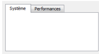
FIGURE 28.21 – QTabWidget
