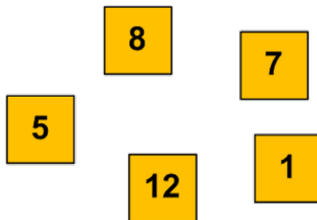
FIGURE 35.6 – set
