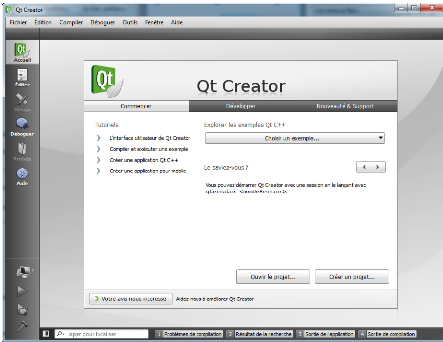
FIGURE 21.12 – Qt Creator
