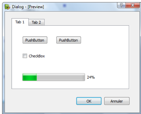
FIGURE 23.10 – Widgets conteneurs
