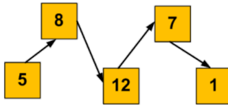
FIGURE 35.4 – list
