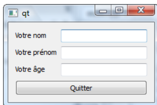
FIGURE 27.20 – Layouts combinés
