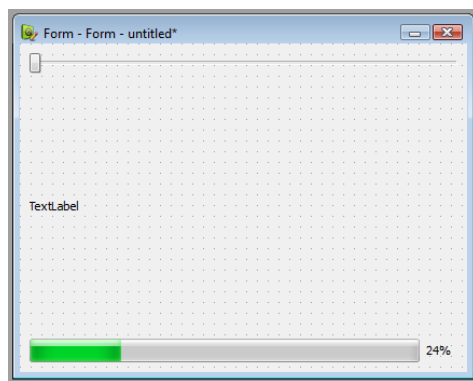
FIGURE 31.7 – Layout vertical
