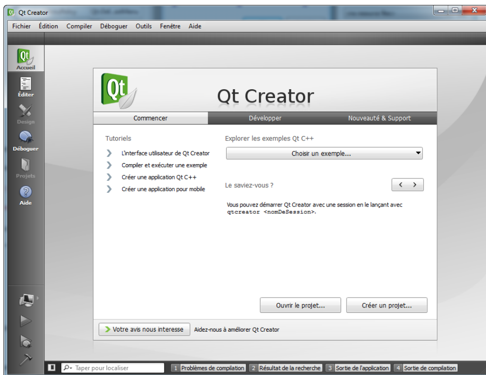
FIGURE 22.1 – Qt Creator
