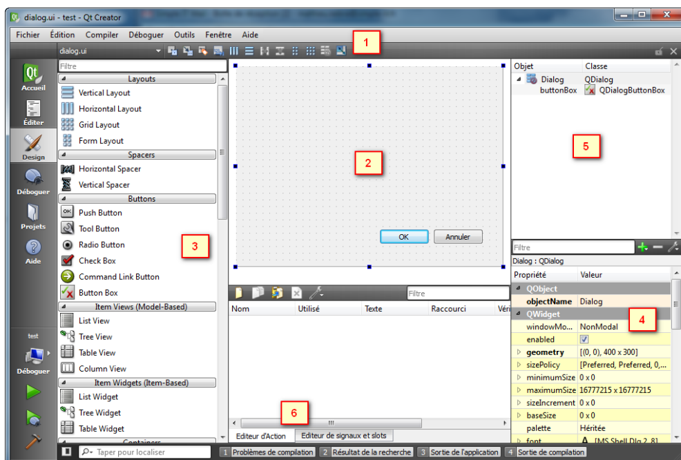
FIGURE 31.4 – Qt Designer dans Qt Creator
