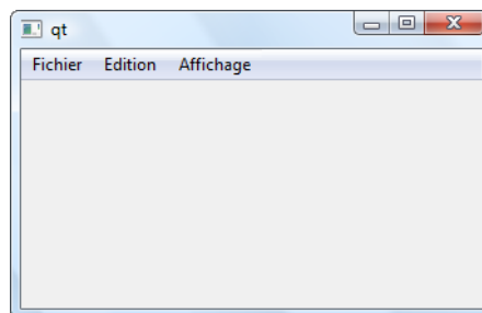
FIGURE 30.6 – Les menus
