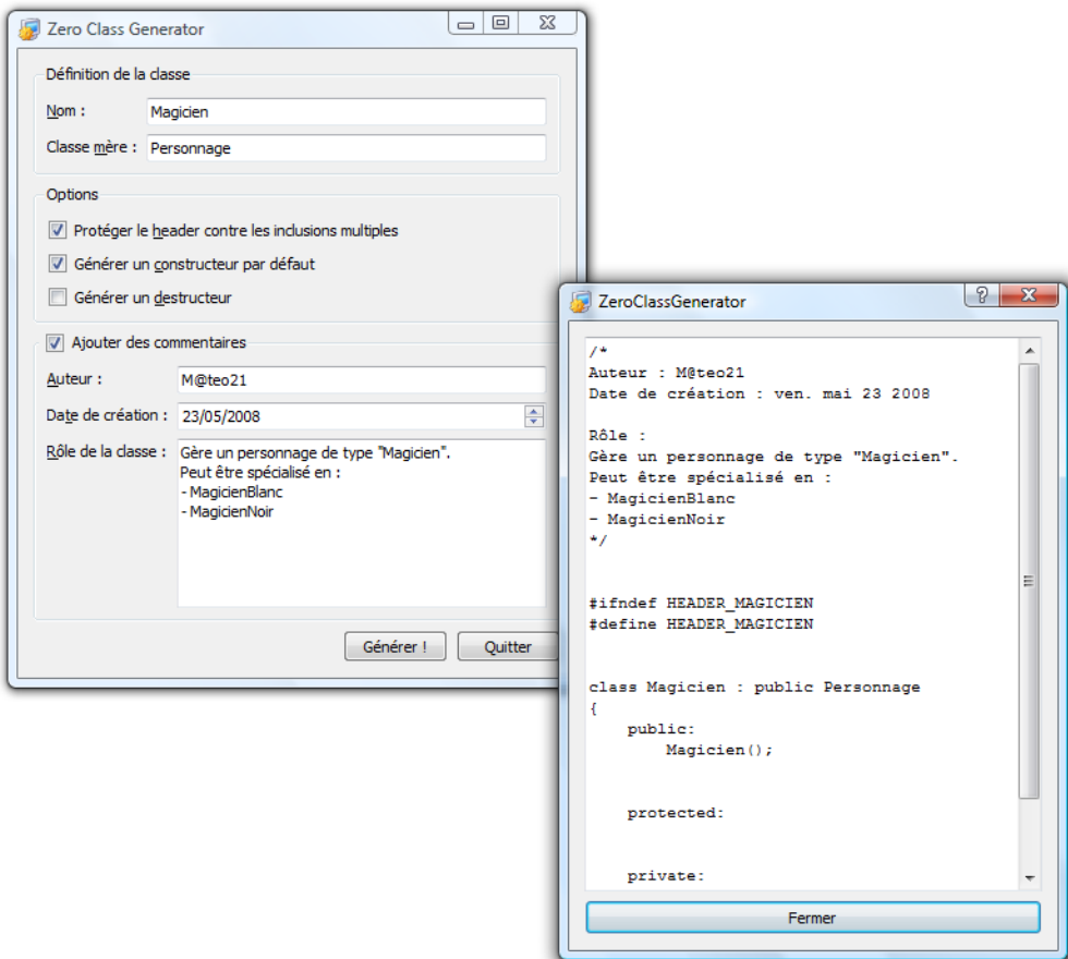
FIGURE 29.1 – Le ZeroClassGenerator
