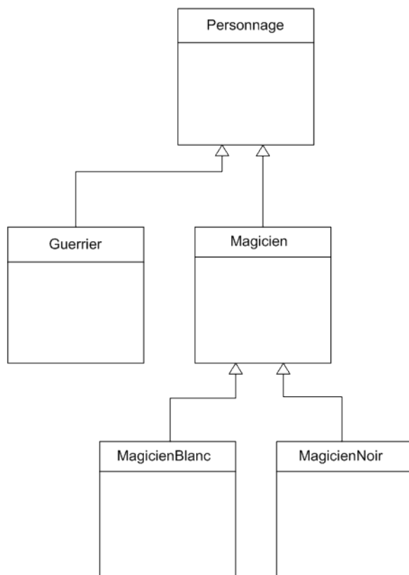
FIGURE 18.3 – Multiples héritages
