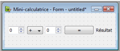
FIGURE 31.16 – Mini-calculatrice
