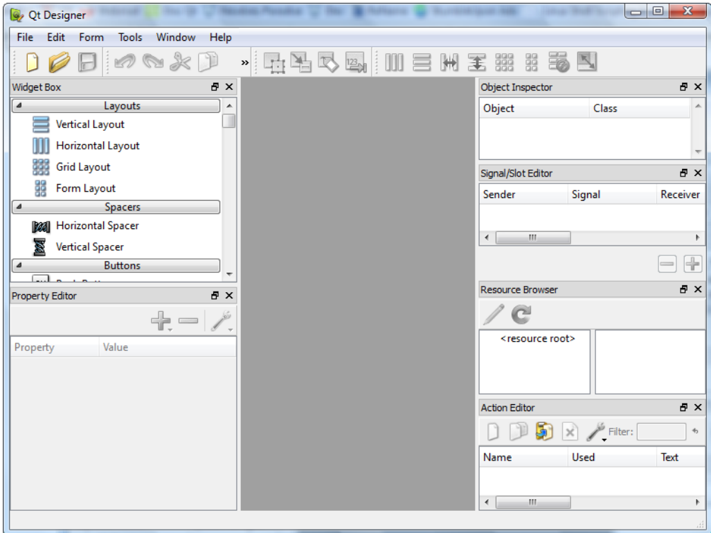
FIGURE 30.2 – Qt Designer et sa QMainWindow
