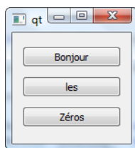
FIGURE 27.8 – Layout vertical
