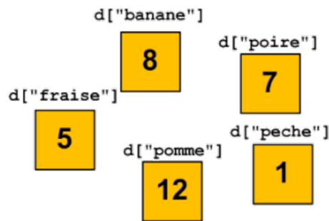
FIGURE 35.5 – map
