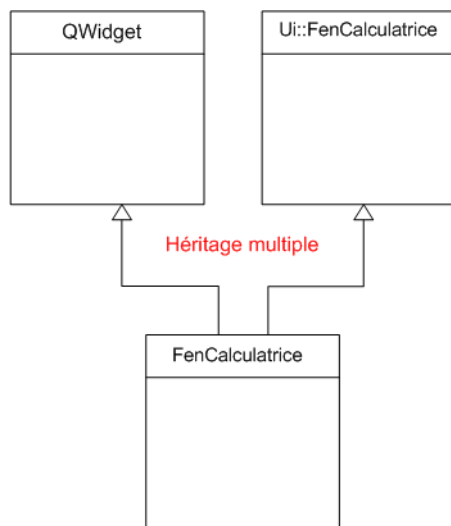
FIGURE 41.1 – Héritage multiple
