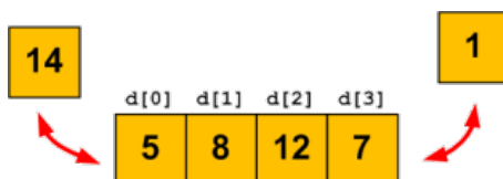
FIGURE 35.3 – deque
