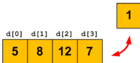
FIGURE 35.2 – vector
