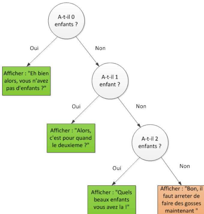
FIGURE 6.2 – Conditions if - else if - else
