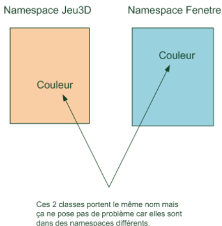
FIGURE 41.2 – Namespaces
