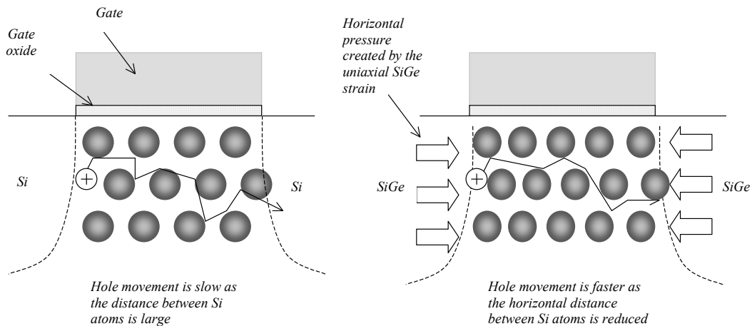
Figure 6: Compressive stain to reduce the distance between atoms underneath the gate, which speeds up the hole mobility of p-channel MOS devices
