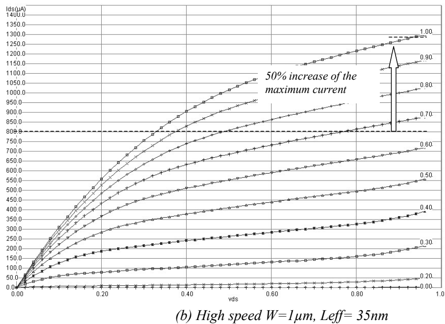
Figure 8: I_d/V_d characteristics of the Low leakage and high speed nMOS devices
