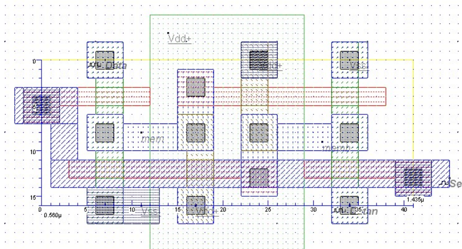
Figure 21: The 6-transistor RAM layout using 65-nm design rules (Ram6T_65nm.MSK)
