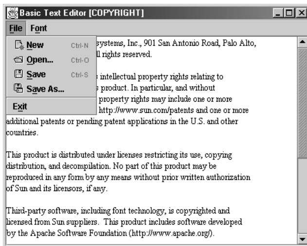
Figure 12.1 Menu containing JMenuItemS with mnemonics and icons
