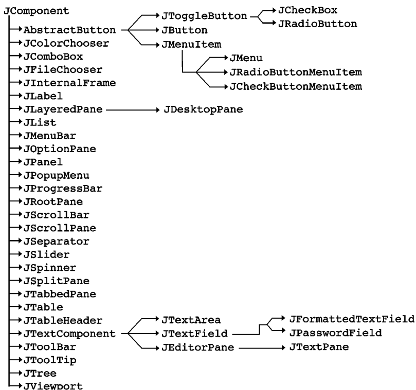
Figure 1.2 Partial JComponent hierarchy
