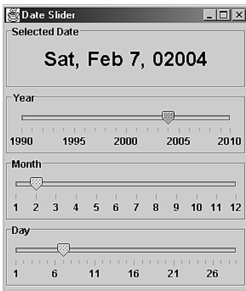
Figure 13.4 JSldiers showing altered maximum bound and annotation labels
