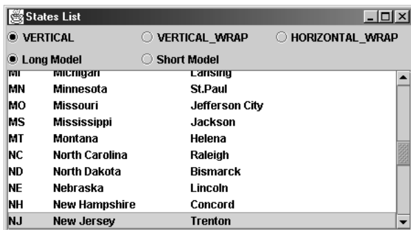
Figure 10.8 A JList that allows accumulated keyboard input to search for a matching item
