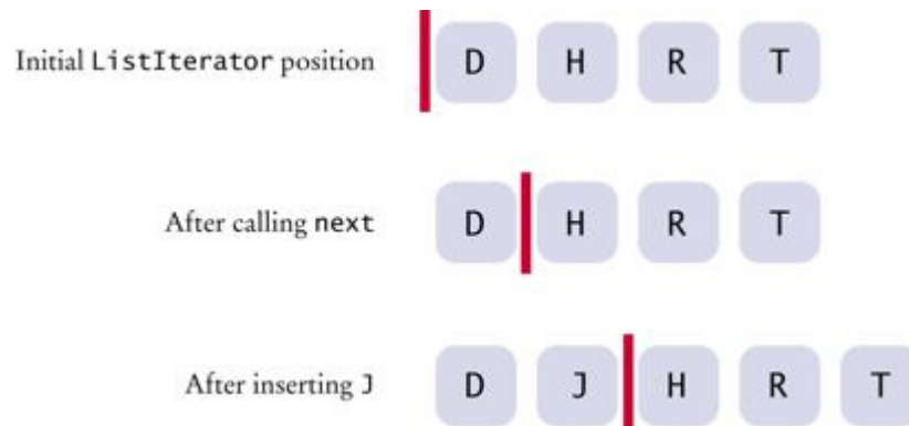
A Conceptual View of the List Iterator
