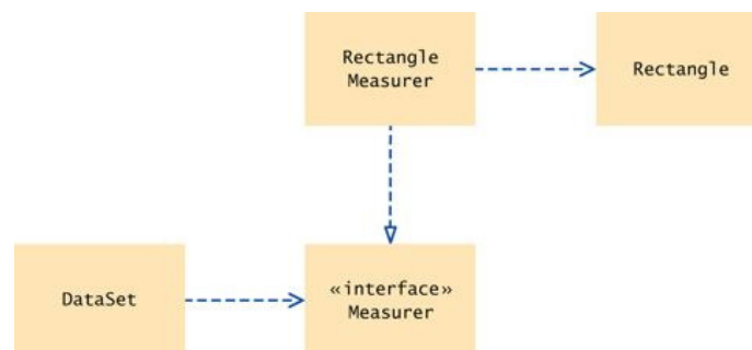
UML Diagram of the DataSet Class and the Measurer Interface
