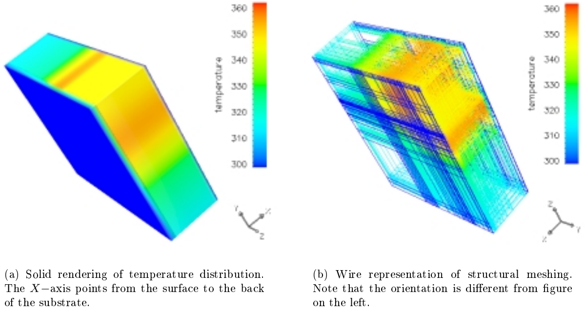
Figure 2: (a) The simulated structure and 3D contour plot for temperature under the specified heat generation condition in Figure 1; (b) Wireframe plot of mesh used in the simulation and the temperature distribution.
