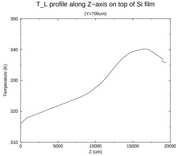
Figure 4: Temperature distribution along the global data path ( X = 7000 \mu\text{m} in Figure 1).
