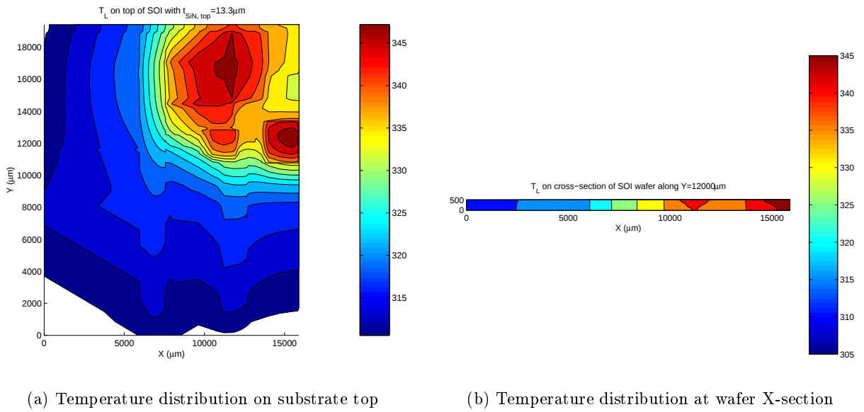
Figure 3: Contour plots for temperature distribution: (a) on the top of the SOI substrate; (b) at the cross-section of the wafer along the line of Y = 12000 \mu\text{m} in Figure 1
