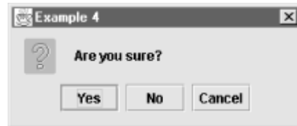
Figure 10.11. Confirm dialog
