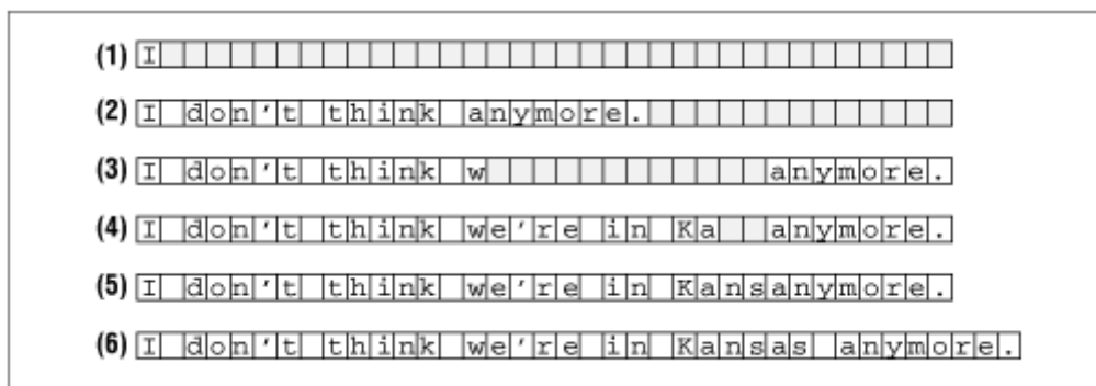
Figure 20.7. GapContent example
