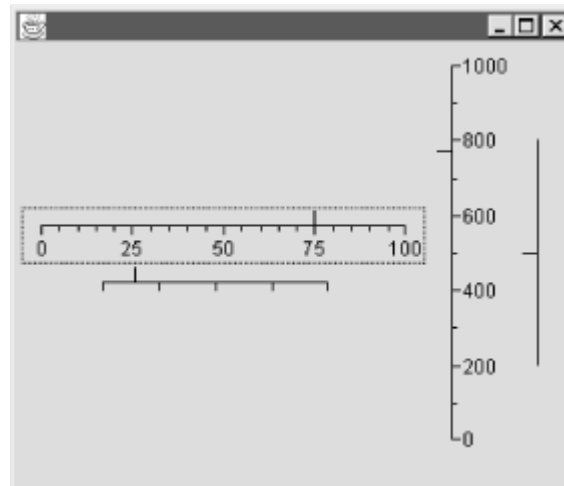
Figure 26.14. PlainSliderUI
