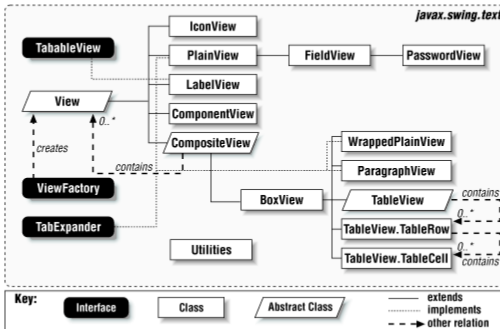
Figure 23.2. View classes
