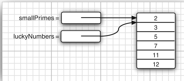
Figure 3.14 Copying an array variable
