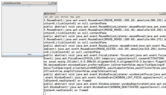
Figure 12.45 The EventTracer class at work
