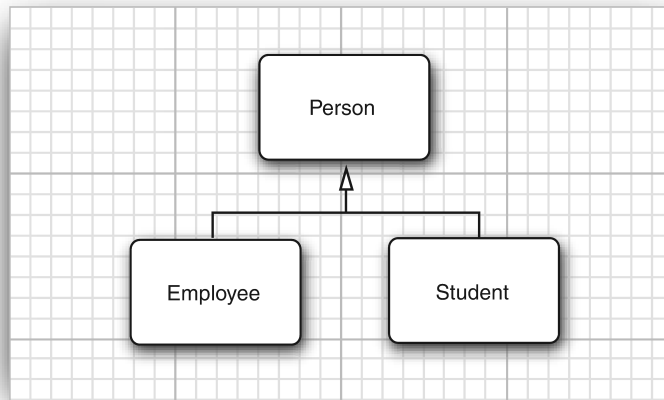
Figure 5.2 Inheritance diagram for Person and its subclasses
