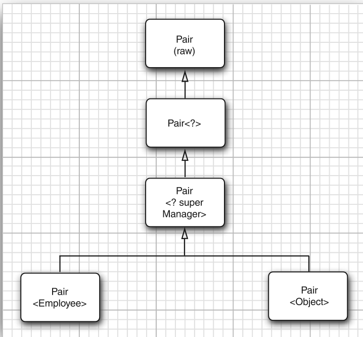
Figure 8.4 A wildcard with a supertype bound
