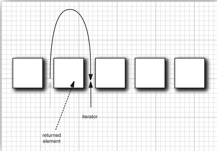
Figure 9.3 Advancing an iterator
