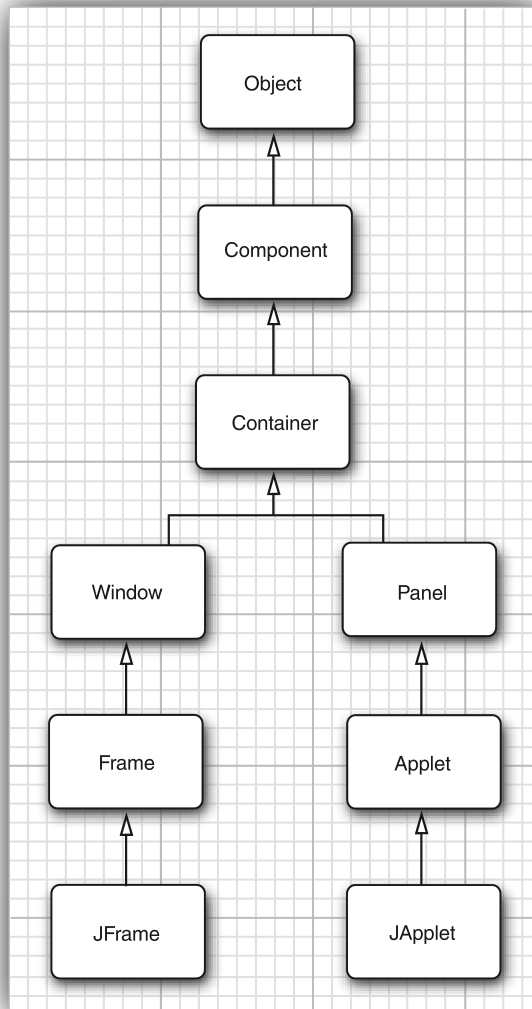
Figure 13.2 Applet inheritance diagram
