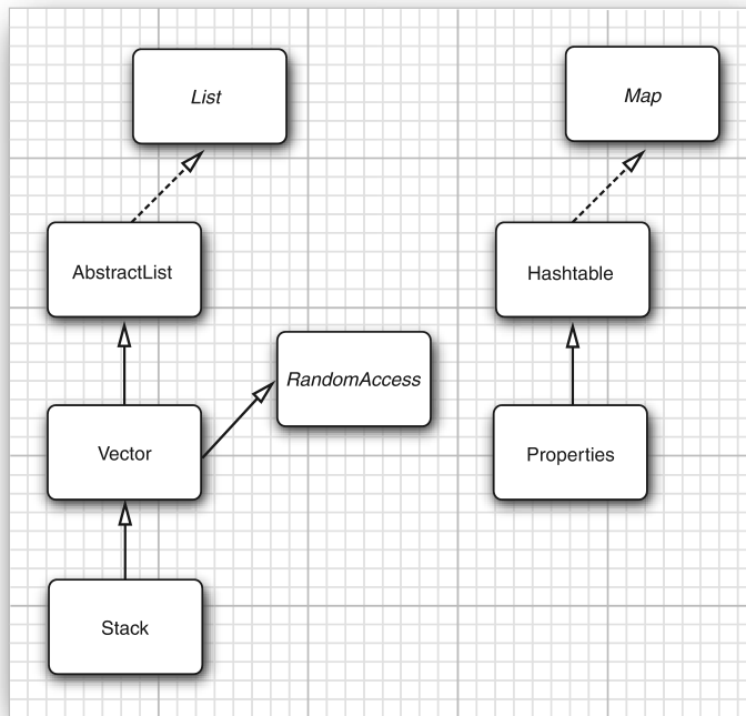
Figure 9.12 Legacy classes in the collections framework
