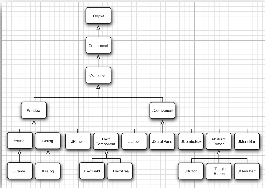
Figure 12.8 Inheritance hierarchy for the Component class
