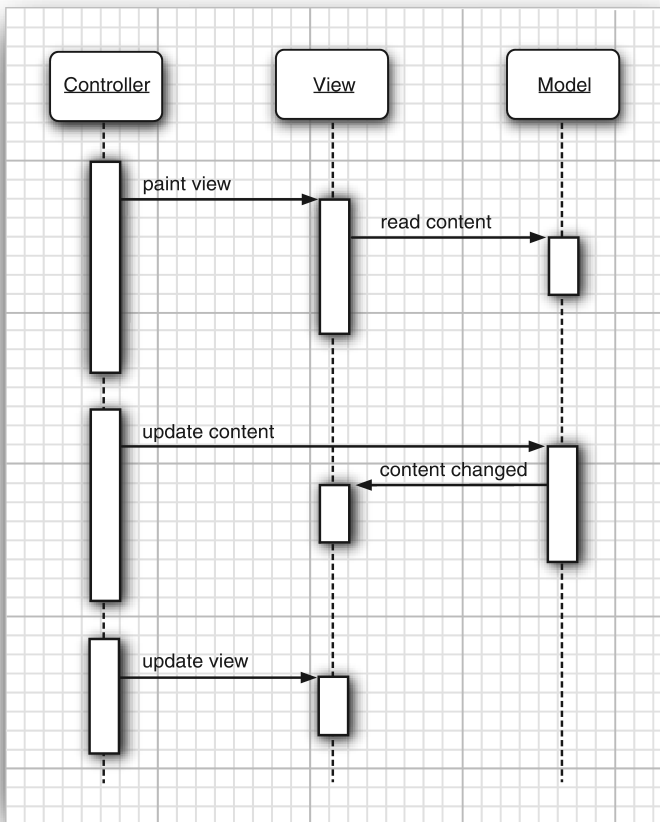
Figure 12.4 Interactions among model, view, and controller objects
