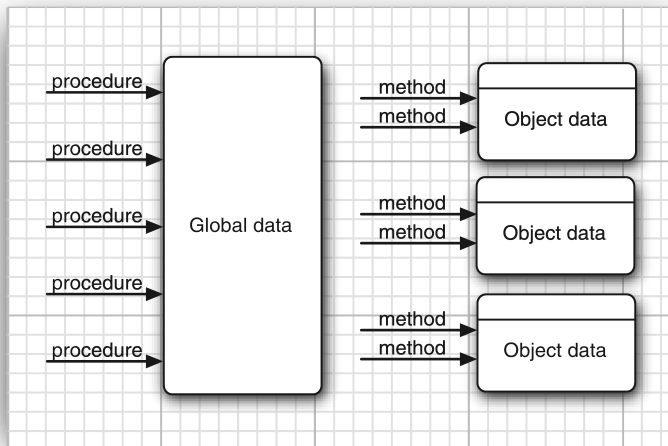
Figure 4.1 Procedural vs. OO programming
