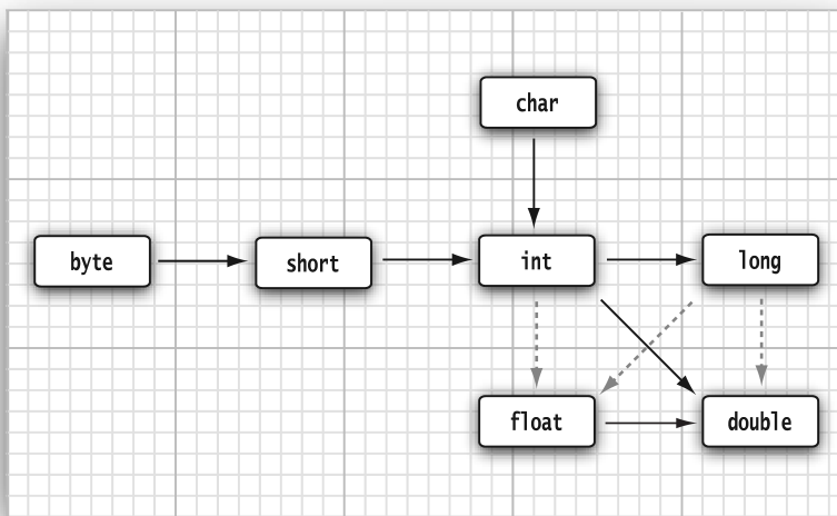
Figure 3.1 Legal conversions between numeric types
