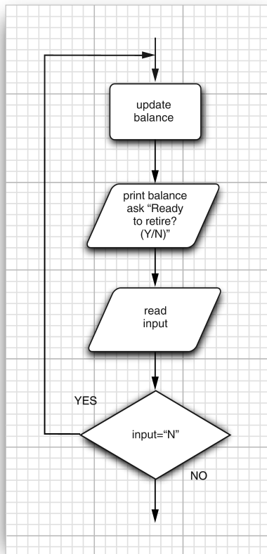
Figure 3.11 Flowchart for the do/while statement
