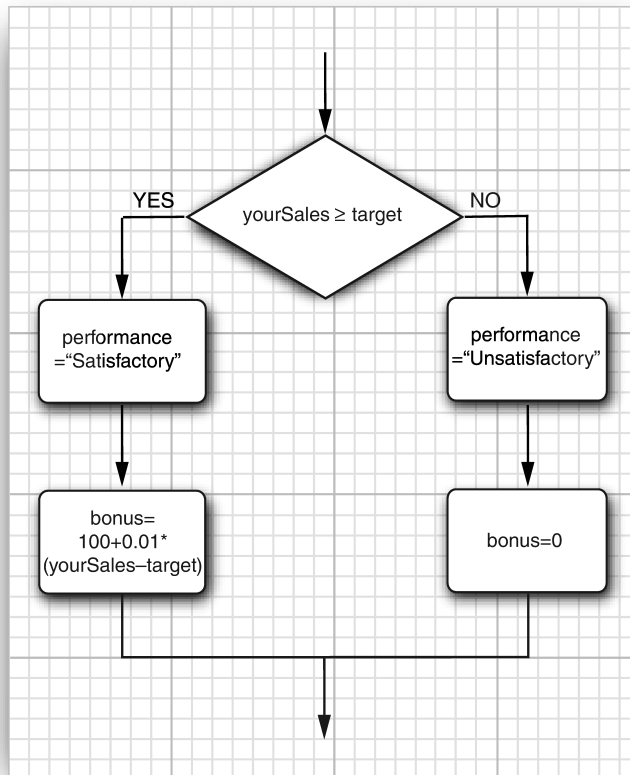
Figure 3.8 Flowchart for the if/else statement
