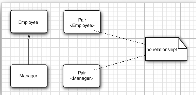
Figure 8.1 No inheritance relationship between pair classes
