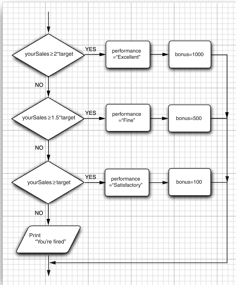
Figure 3.9 Flowchart for the if/else if (multiple branches)
