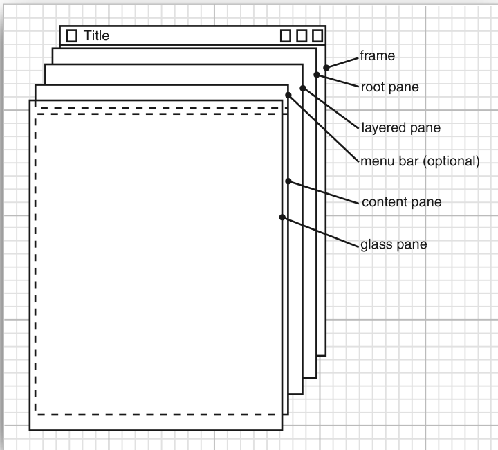
Figure 10.8 Internal structure of a JFrame
