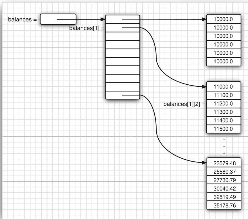
Figure 3.15 A two-dimensional array
