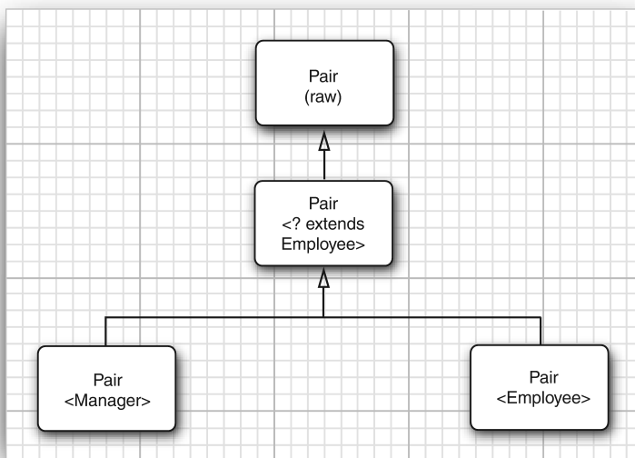
Figure 8.3 Subtype relationships with wildcards
