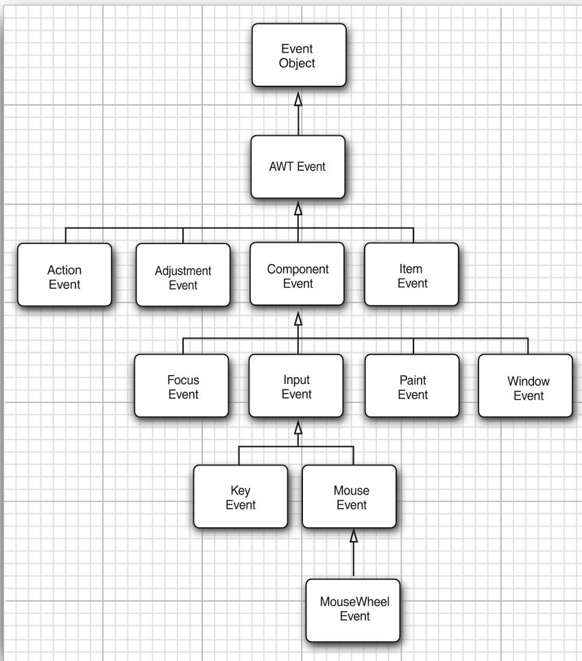
Figure 11.8 Inheritance diagram of AWT event classes
