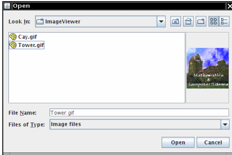
Figure 12.41 A file dialog with a preview accessory
