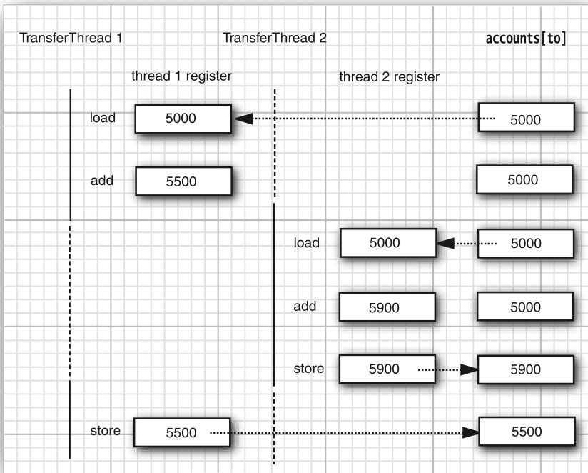
Figure 14.4 Simultaneous access by two threads
