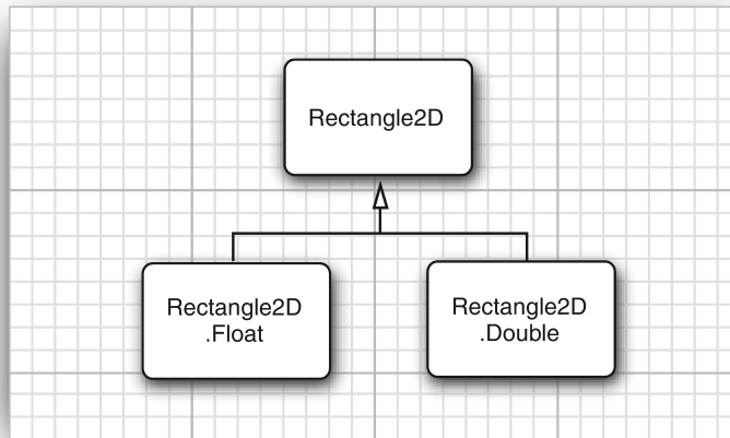
Figure 10.9 2D rectangle classes
