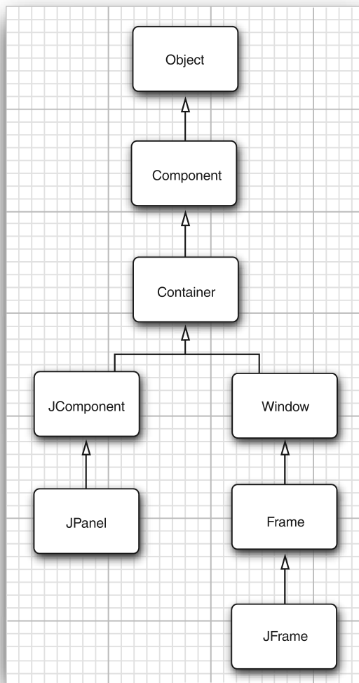
Figure 10.6 Inheritance hierarchy for the frame and component classes in AWT and Swing
