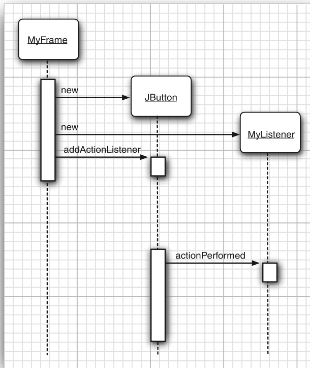
Figure 11.2 Event notification
