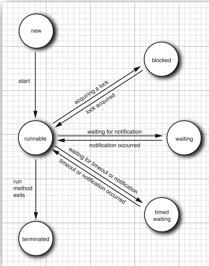
Figure 14.3 Thread states
