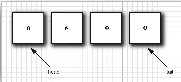
Figure 9.1 A queue
