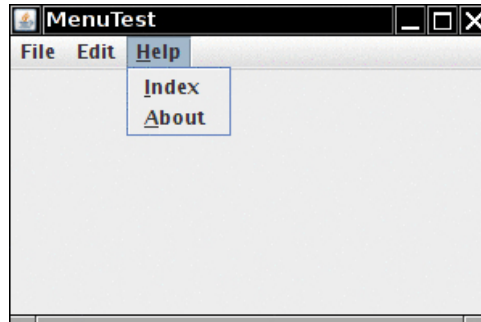
Figure 12.21 Keyboard mnemonics
