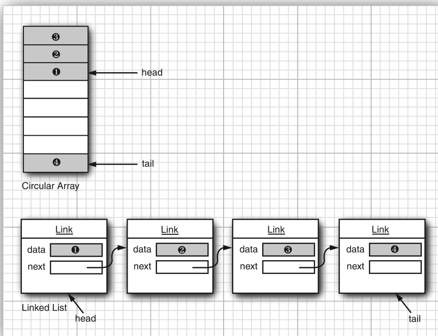
Figure 9.2 Queue implementations
