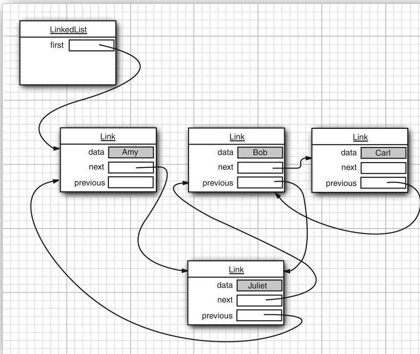
Figure 9.9 Adding an element to a linked list
