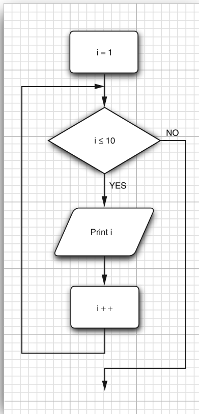
Figure 3.12 Flowchart for the for statement
