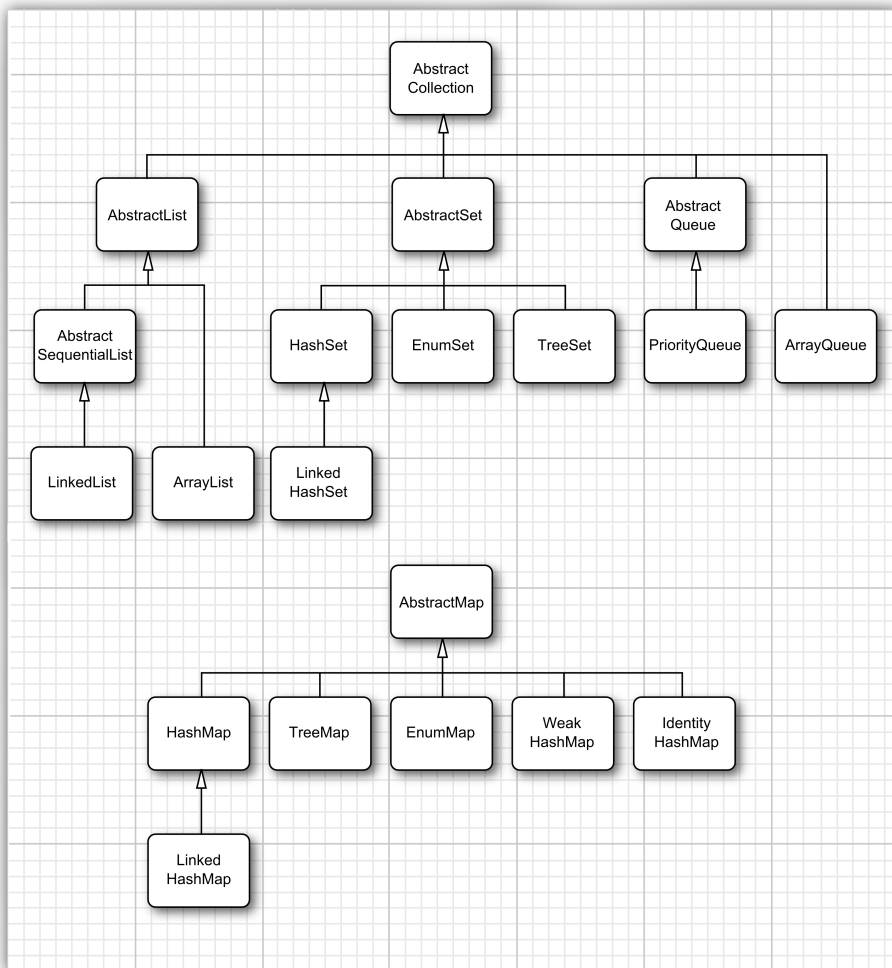
Figure 9.5 Classes in the collections framework
