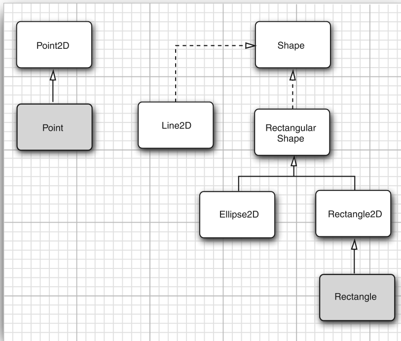
Figure 10.11 Relationships between the shape classes
