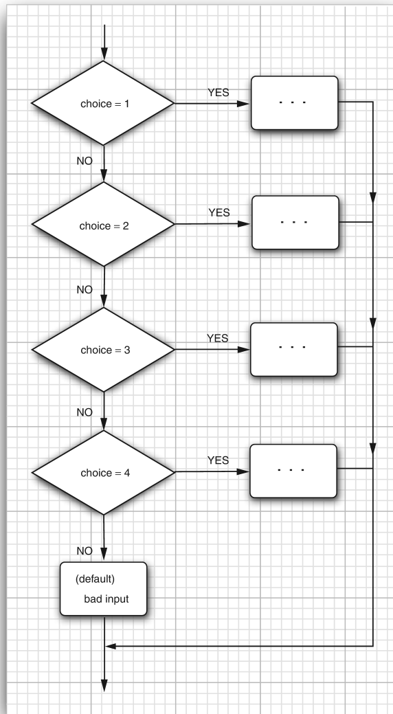
Figure 3.13 Flowchart for the switch statement
