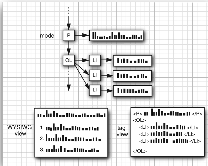
Figure 12.3 Two separate views of the same model
