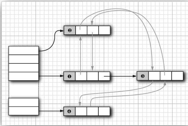
Figure 9.11 A linked hash table
