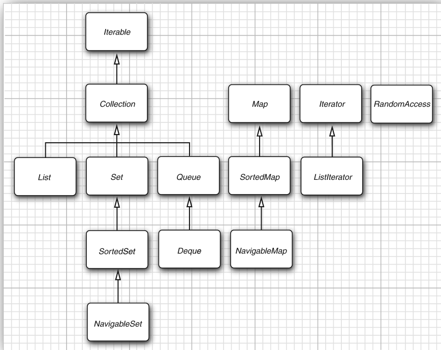
Figure 9.4 The interfaces of the collections framework
