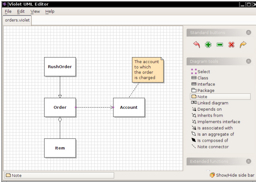
Figure 4.2 A class diagram
