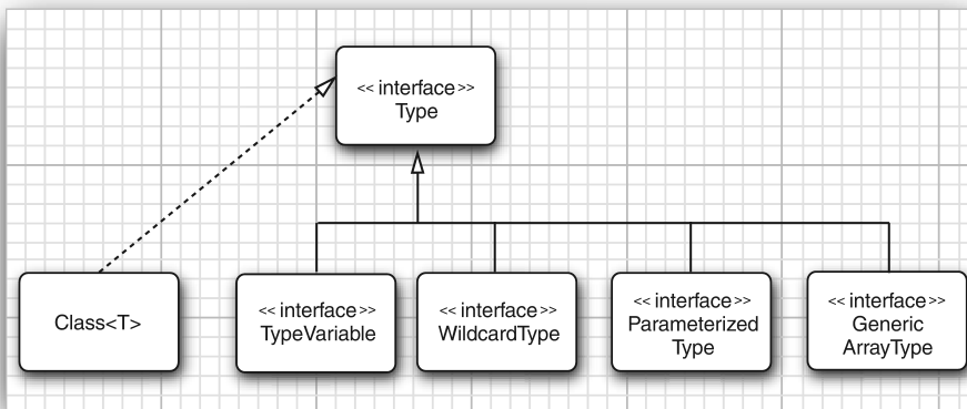
Figure 8.5 The Type interface and its descendants
