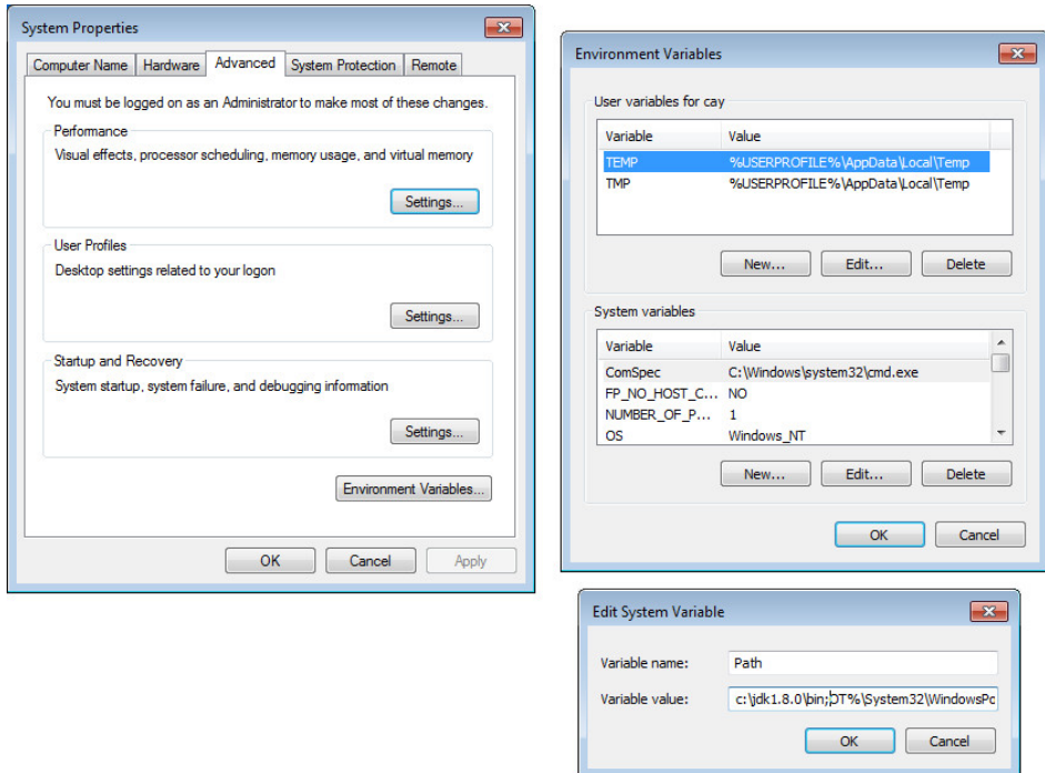
Figure 2.2 Setting the Path environment variable in Windows 7
