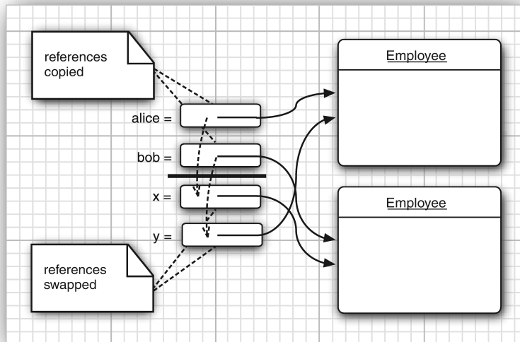
Figure 4.8 Swapping object parameters has no lasting effect.
