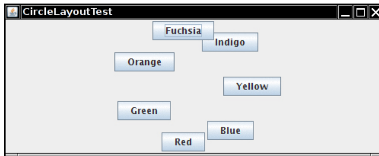
Figure 12.34 Circle layout
