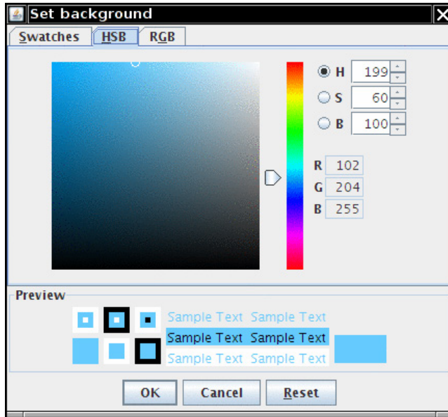
Figure 12.43 The HSB pane of a color chooser
