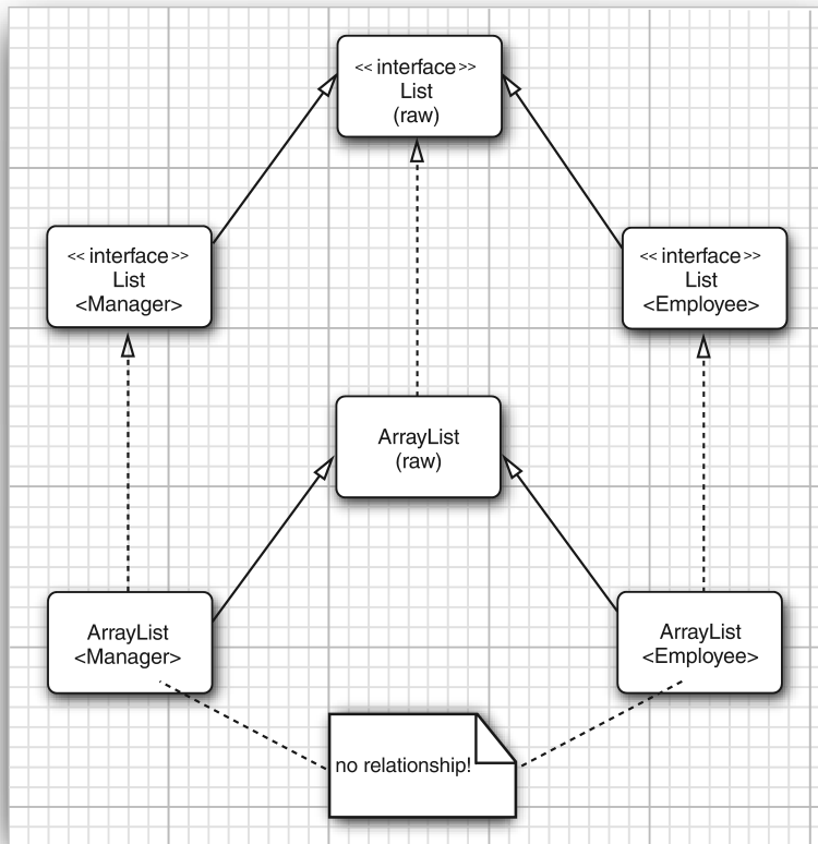
Figure 8.2 Subtype relationships among generic list types
