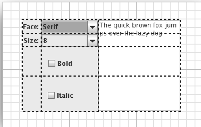
Figure 12.30 Dialog box grid used in design
