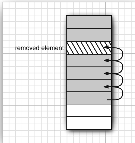
Figure 9.6 Removing an element from an array
