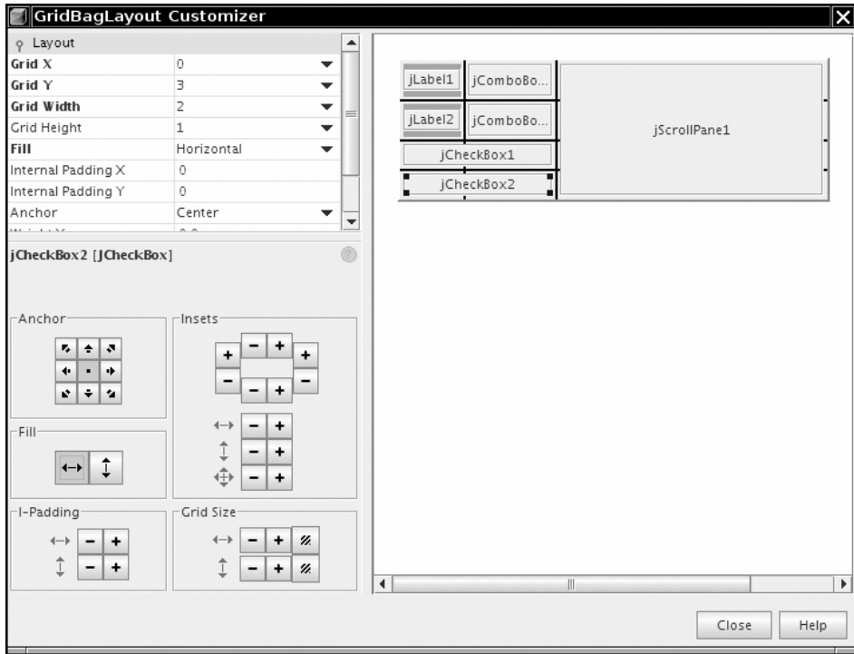
Figure 12.31 Specifying grid bag constraints in NetBeans
