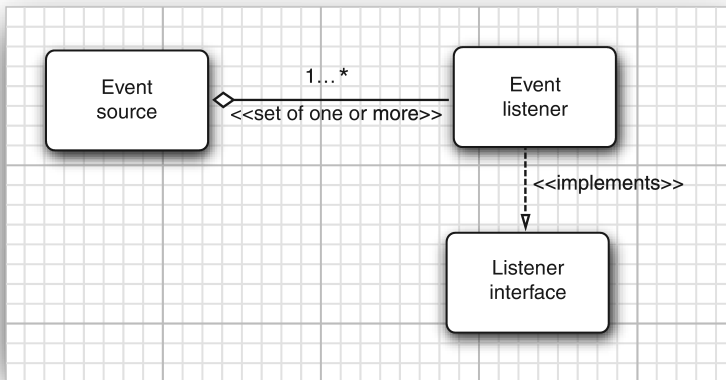
Figure 11.1 Relationship between event sources and listeners
