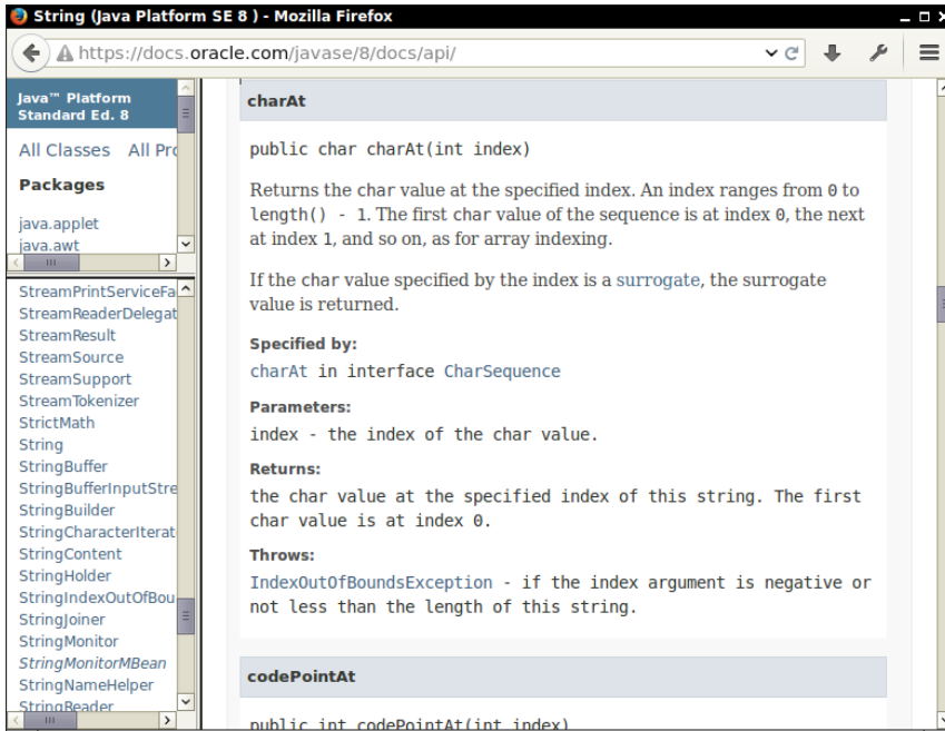
Figure 3.5 Detailed description of a String method
