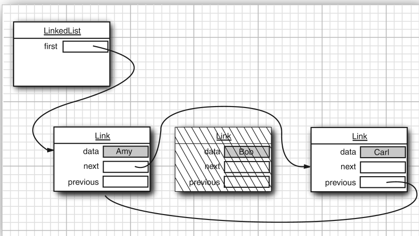
Figure 9.8 Removing an element from a linked list
