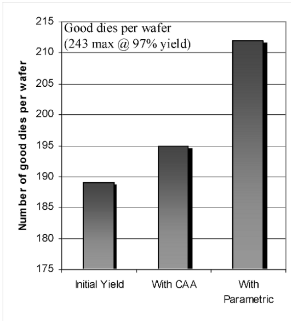
Figure 1-6. DfY techniques improve yield [54].
