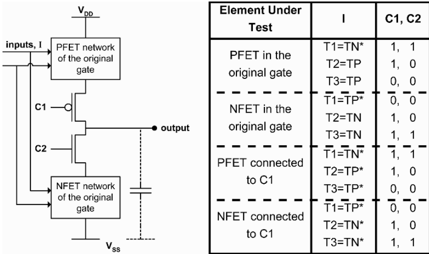
Figure 3-7. Robust SOP fault detection scheme and the 3-pattern test procedure [74].
