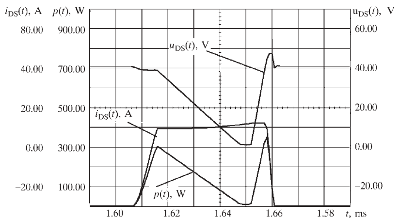
Fig. 4 Simulated characteristic TEMPFET's waveforms for combined losses operating conditions using electro-thermal model
