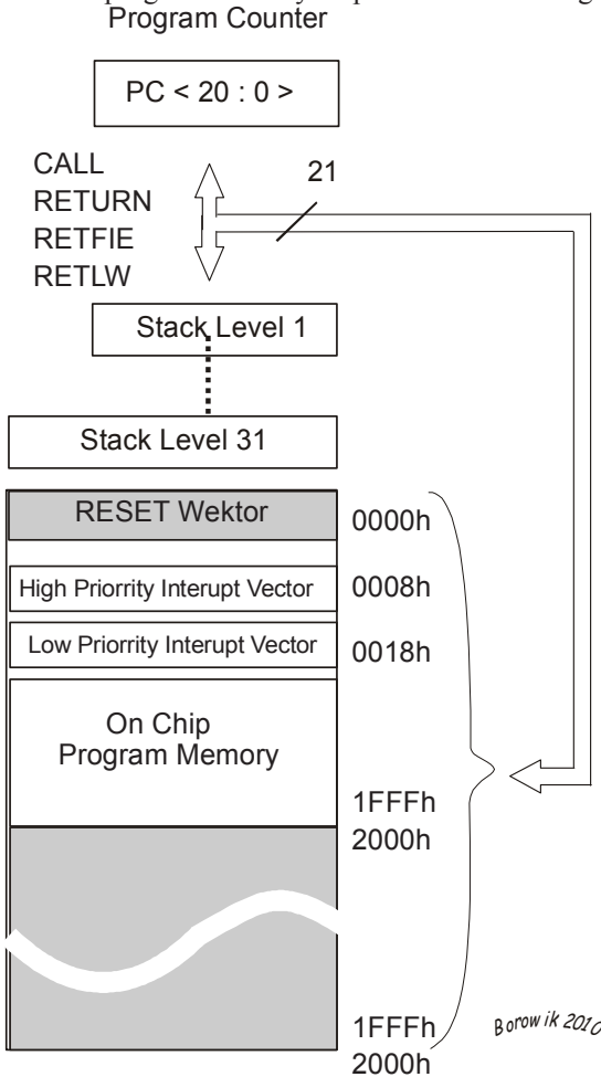
Fig.35. Program memory map and stack for PIC18F1320
