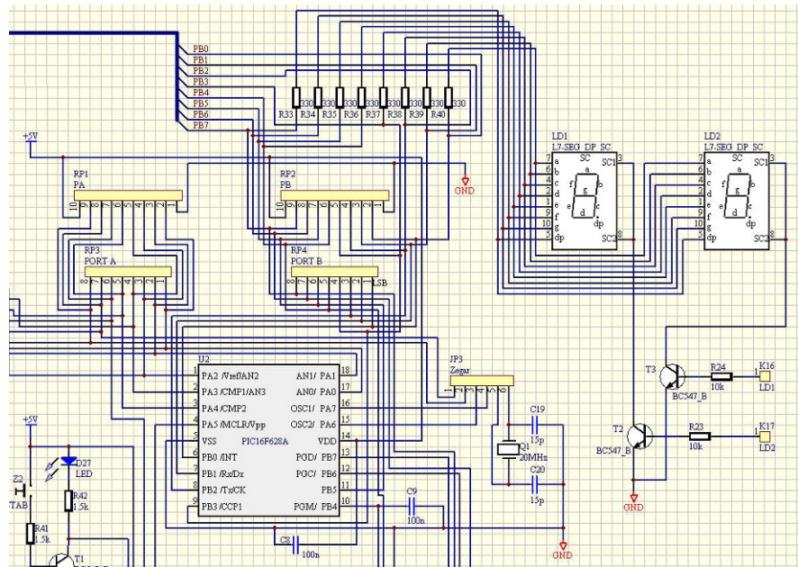
Fig. 2. 7-Segment Display connected to port B
