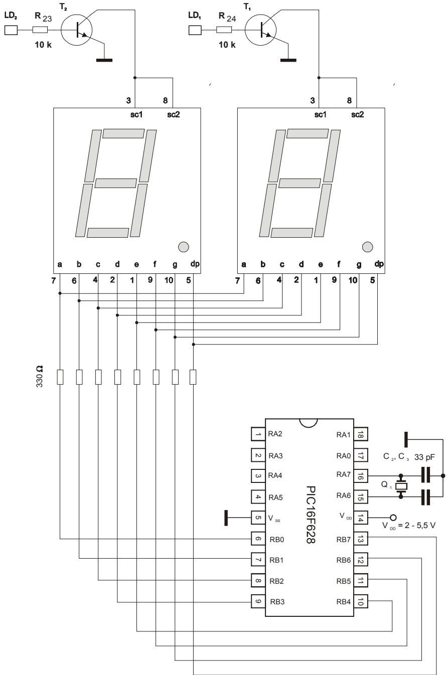
Fig. 24 Connecting a microcontroller to 7-segment display
