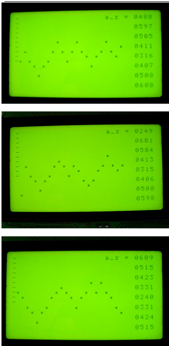
Fig.44 Scattergram with data from accelerometer
