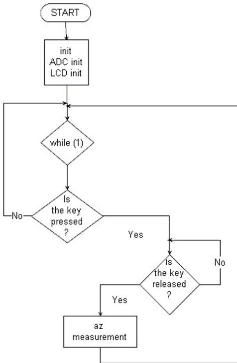
Fig.45 Application flowchart nr 1
