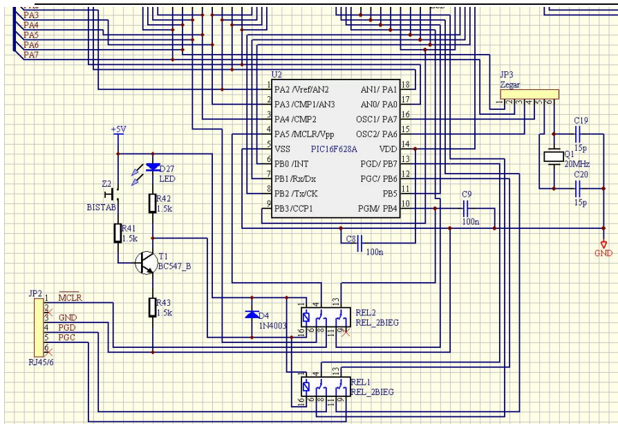
Fig. 1. In Circuit Serial Programming ICSP device connected to JP2
