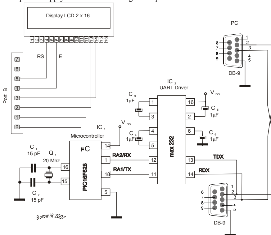
Fig. 32 Schematic diagram for TX/RX operations
