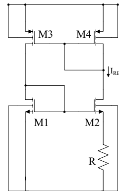
Fig. 4. PTAT current reference.
