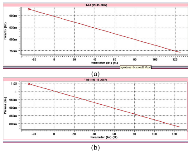
Fig. 3. Threshold voltage versus temperature characteristic curve of MXIC 0.5 \mu m technology for: (a) NMOS and (b)PMOS
