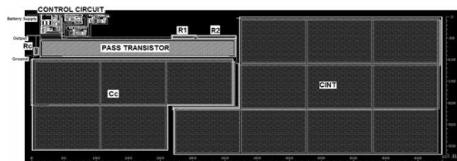
Fig. 13 Layout for the proposed LDO voltage regulator
