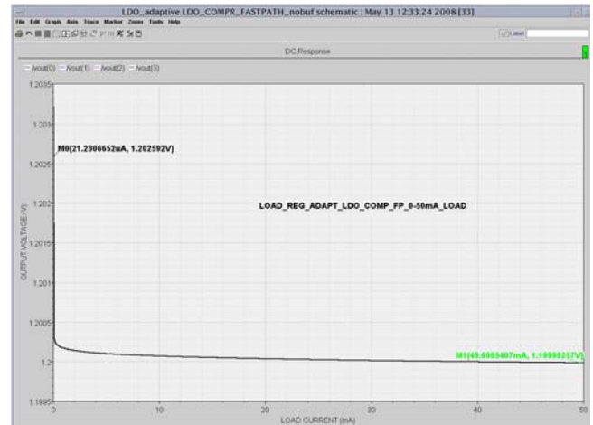
Fig. 12 Load regulation of the proposed LDO with load current varying from 0-50mA
