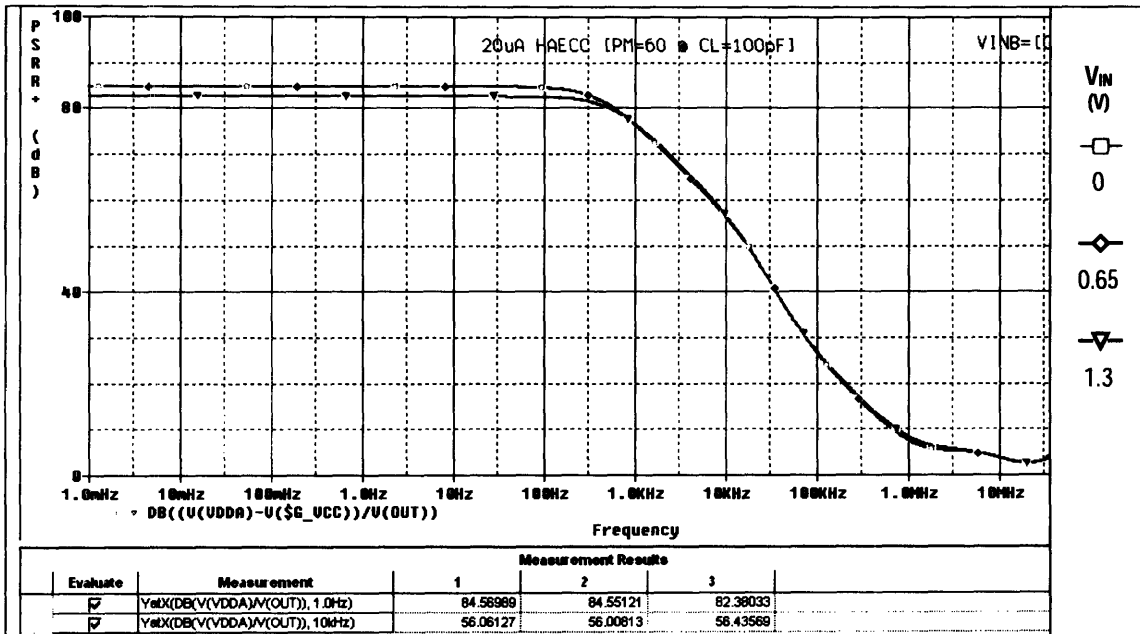
Figure D-5: PSRR+ vs Frequency with V_{IN}=0, 0.65, 1.3V
