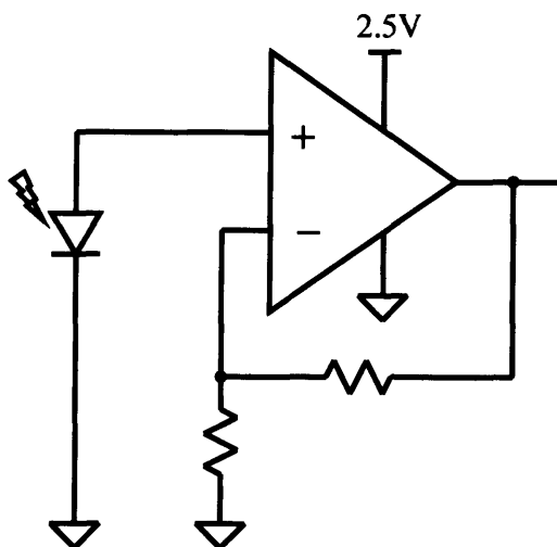
Figure 1-1: Photodiode Amplifier with Single-supply
