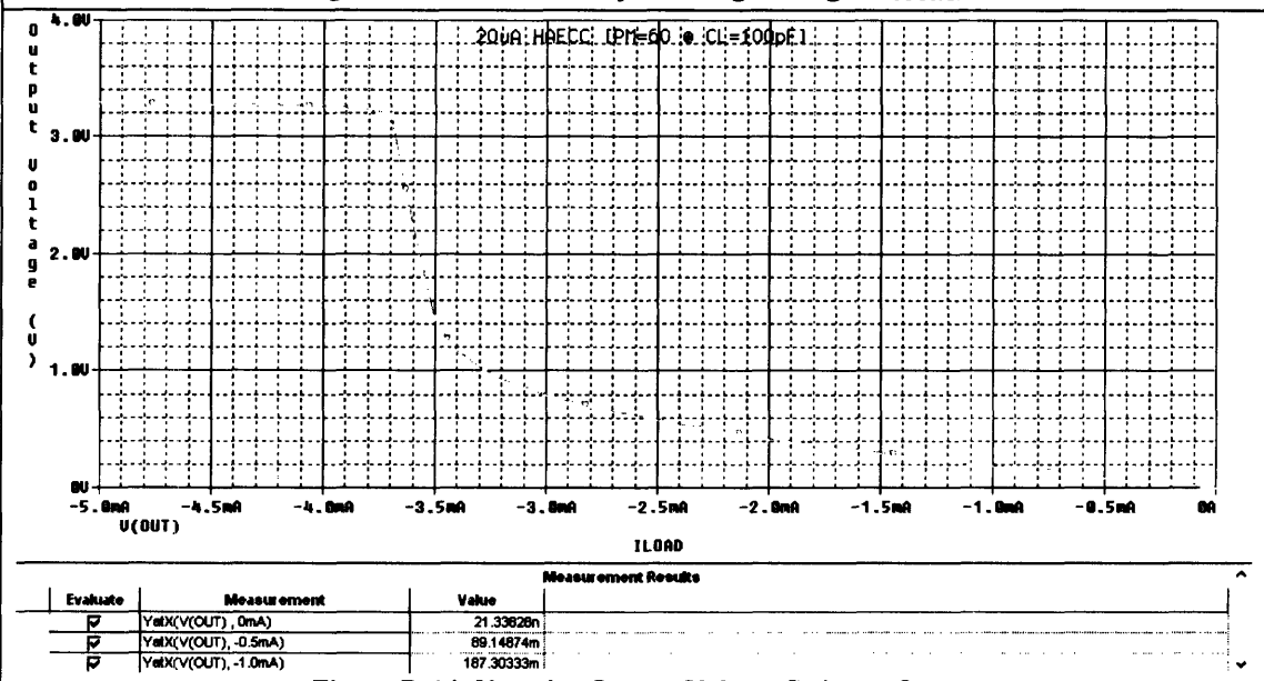
Figure D-14: Negative Output Voltage Swing vs I_{SINK}
