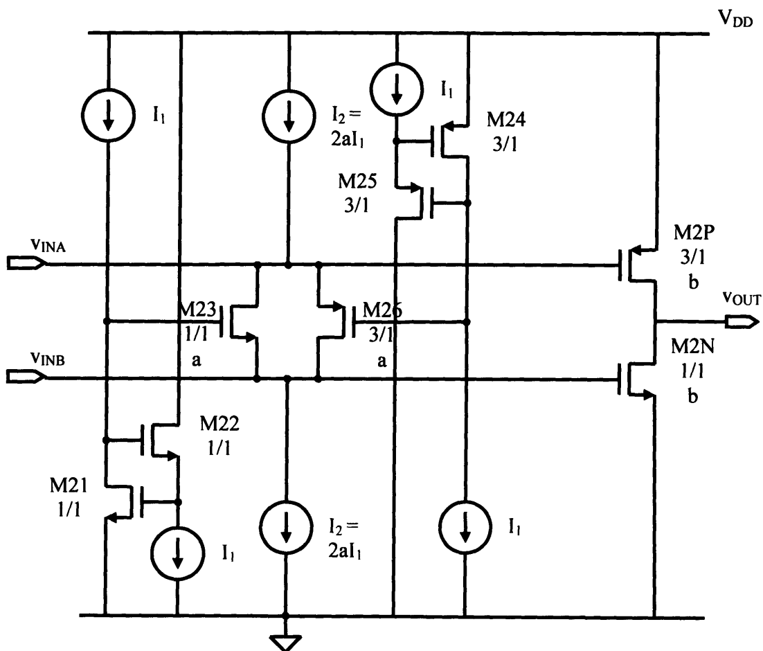
Figure 3-5: Modified Translinear-Loop-Biased Class AB Output Stage
