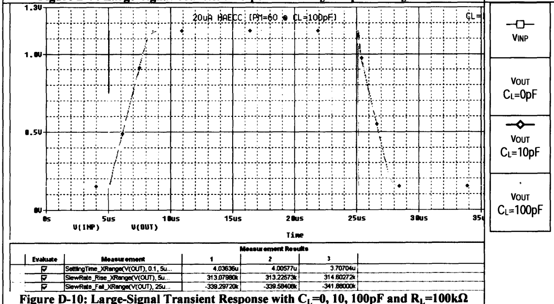
Figure D-10: Large-Signal Transient Response with C_L=0, 10, 100\text{pF} and R_L=100\text{k}\Omega
