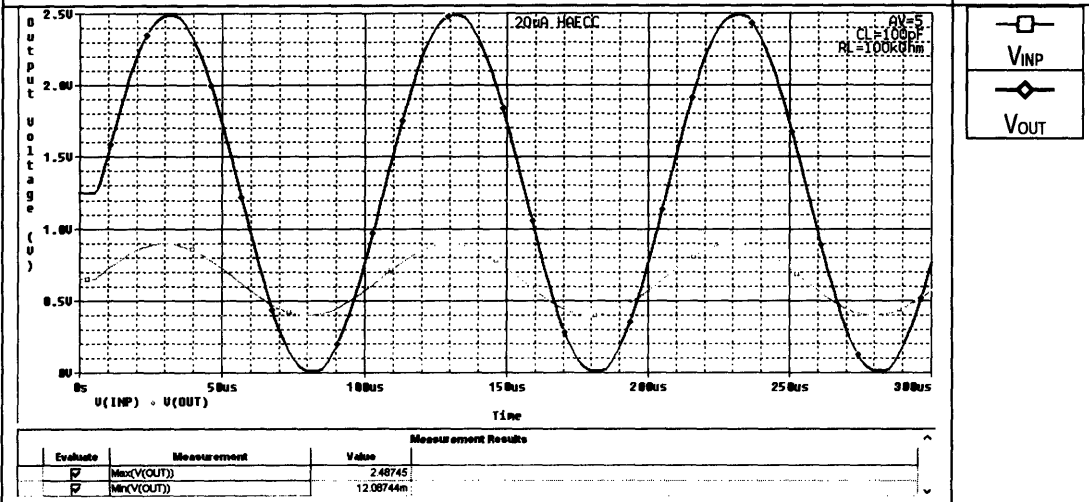
Figure D-12: Rail-to-Rail Output Voltage ( V_{IN} and V_{OUT} with A_V=5 )
