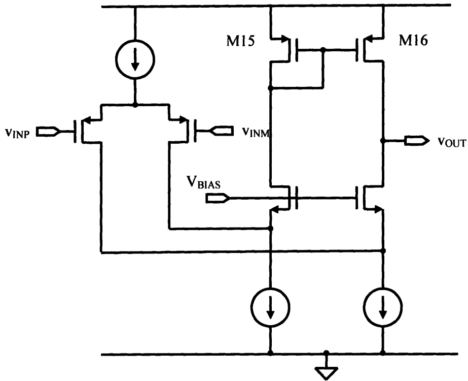
Figure 2-3: Folded-Cascode Input Stage (adapted from [9] to have the PMOS input pair)
