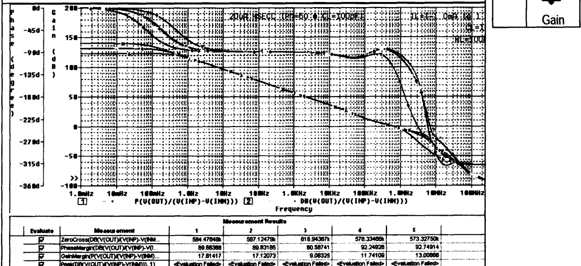
Figure C-19: Frequency Response with C_L=100pF and R_L=100k\Omega @ I_L=-1.0, -0.5, 0.0, 0.5, 1.0mA
