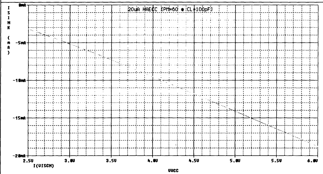
Figure D-16: Short-Circuit Sink Current vs Supply Voltage
