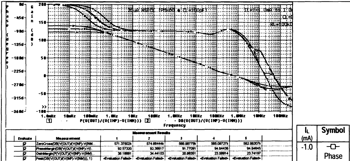
Figure C-17: Frequency Response with C_L=0pF and R_L=100k\Omega @ I_L=-1.0, -0.5, 0.0, 0.5, 1.0mA
