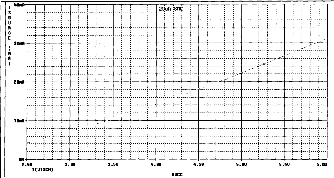
Figure A-15: Short-Circuit Source Current vs Supply Voltage
