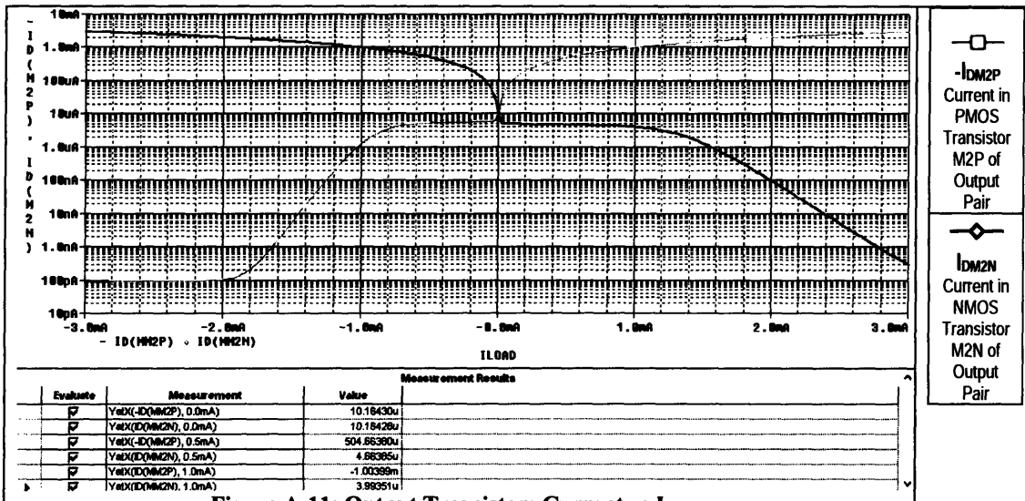
Figure A-11: Output Transistors Current vs I_{LOAD}
