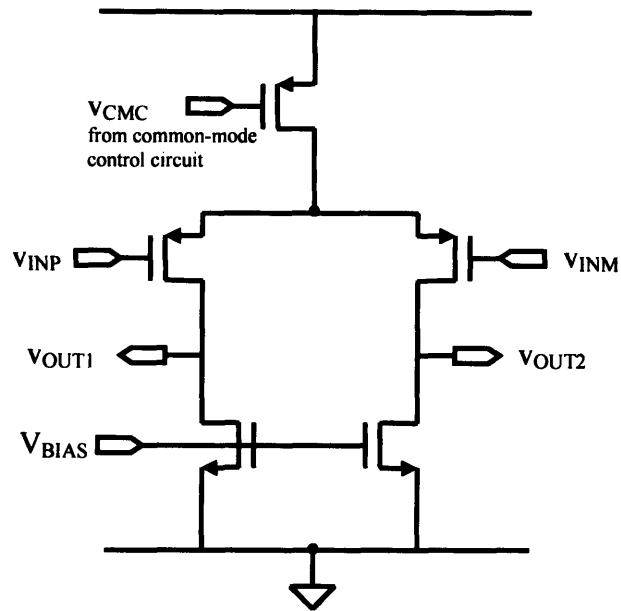
Figure 2-2: Fully Differential Basic Input Stage [8]
