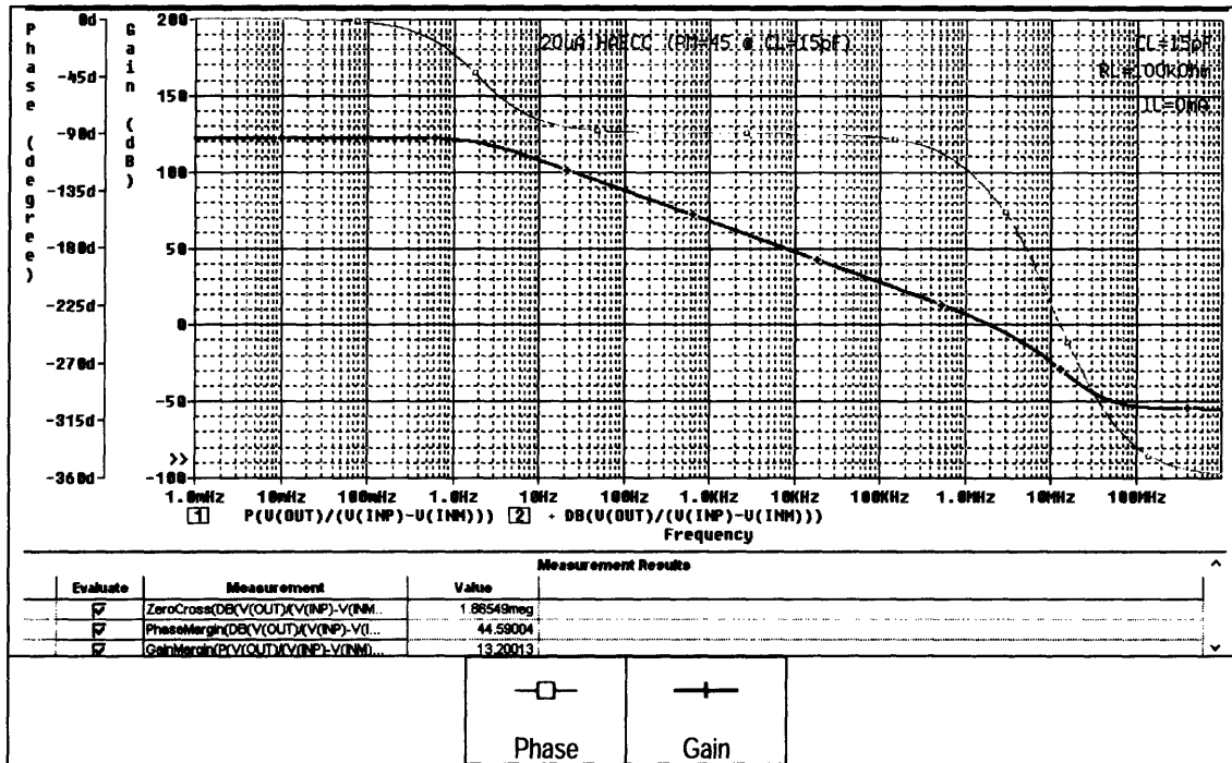
Figure 6-1: Frequency Response of 20μA Micropower Op Amp with HAECC Compensated Down to Have \Phi_M = 45^\circ at 15pF Load to Compare with MAX9914
