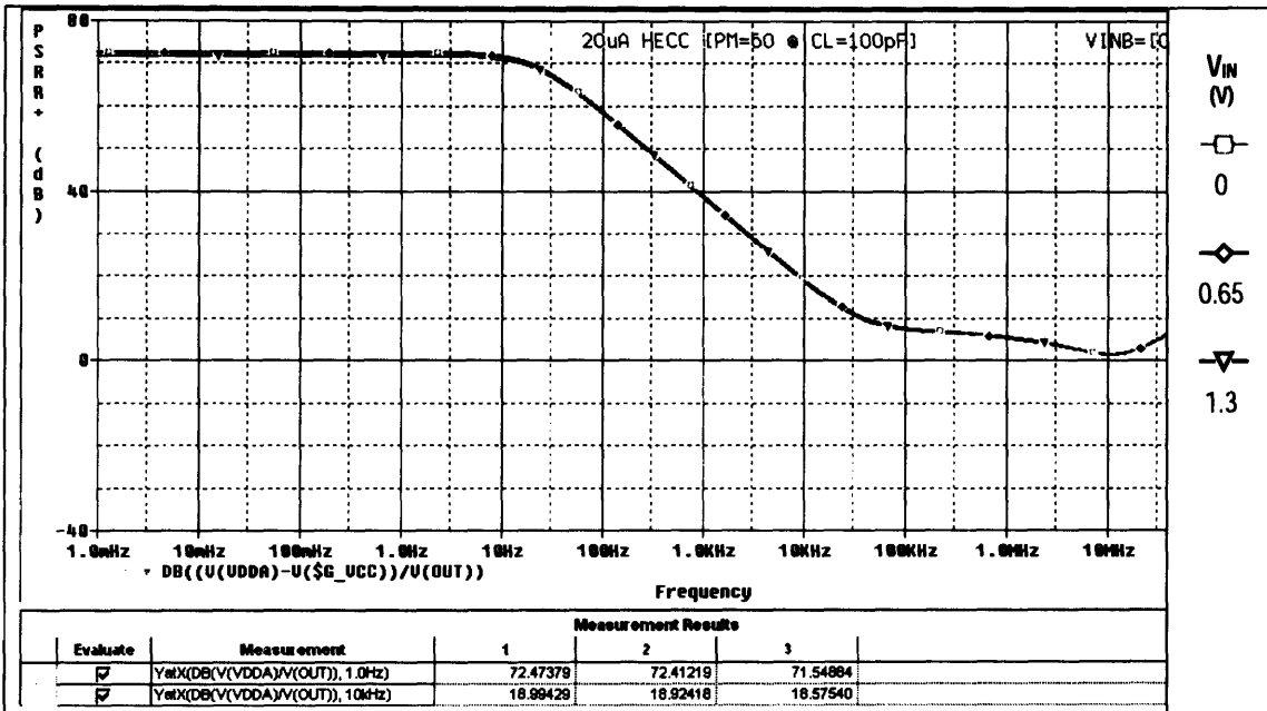
Figure B-5: PSRR+ vs Frequency with V_{IN}=0, 0.65, 1.3V
