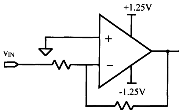
Figure 1-2: Inverting Amplifier with Dual Supplies
