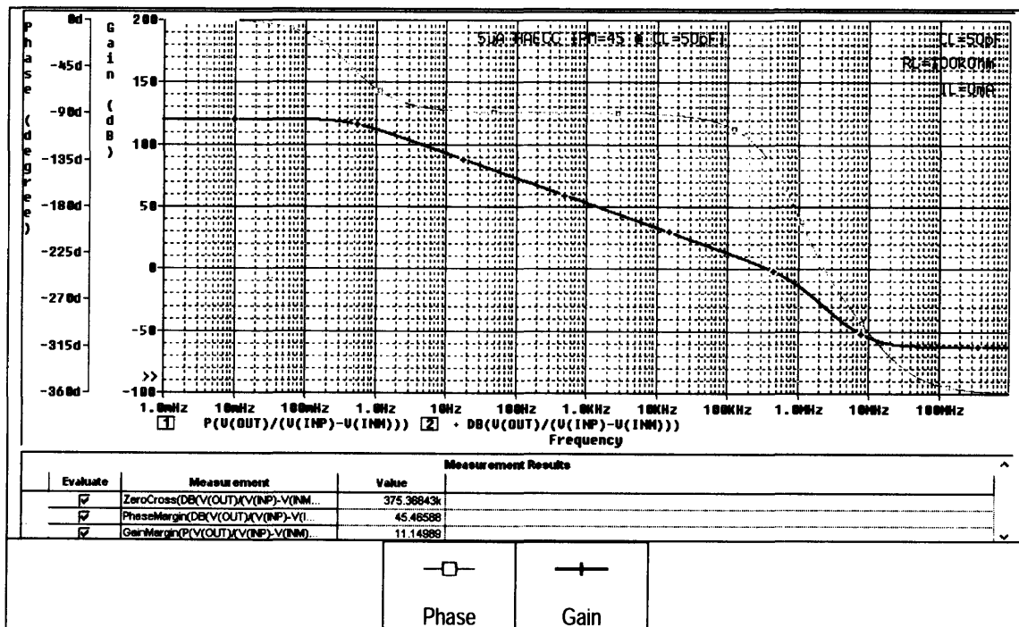
Figure 6-2: Frequency Response of 5 \mu A Micropower Op Amp with HAECC Compensated Down to Have \Phi_M = 45^\circ at 50pF Load to Compare with MIC861
