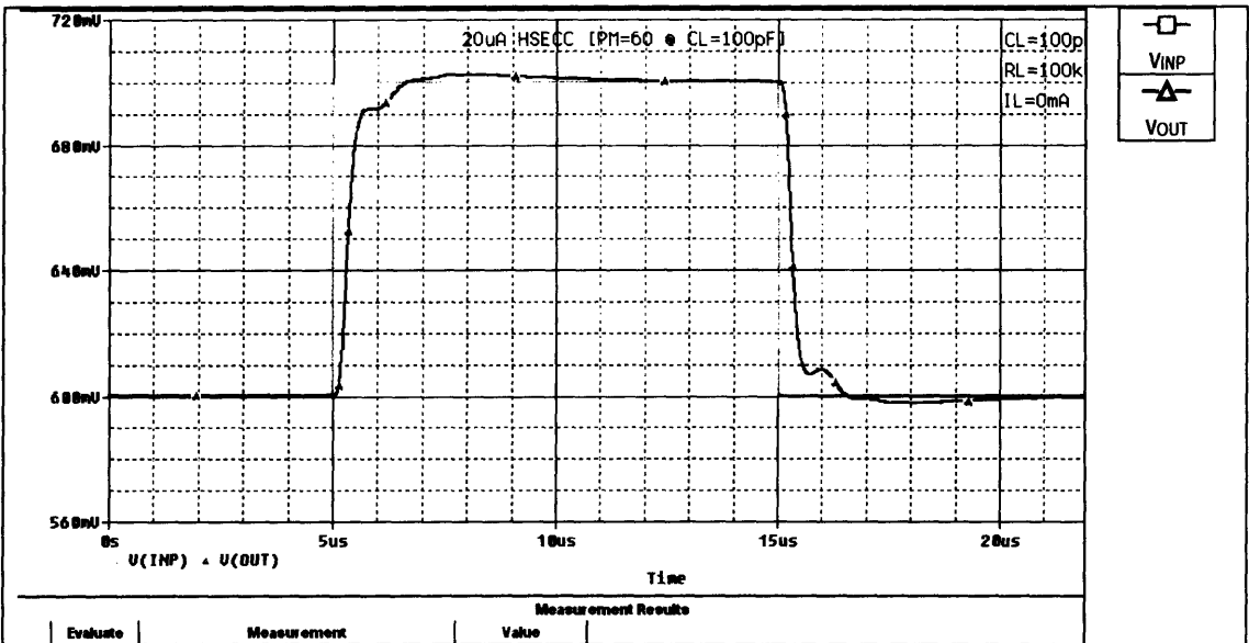
Figure C-7: Small-Signal Transient Response with C_L=100\text{pF} and R_L=100\text{k}\Omega
