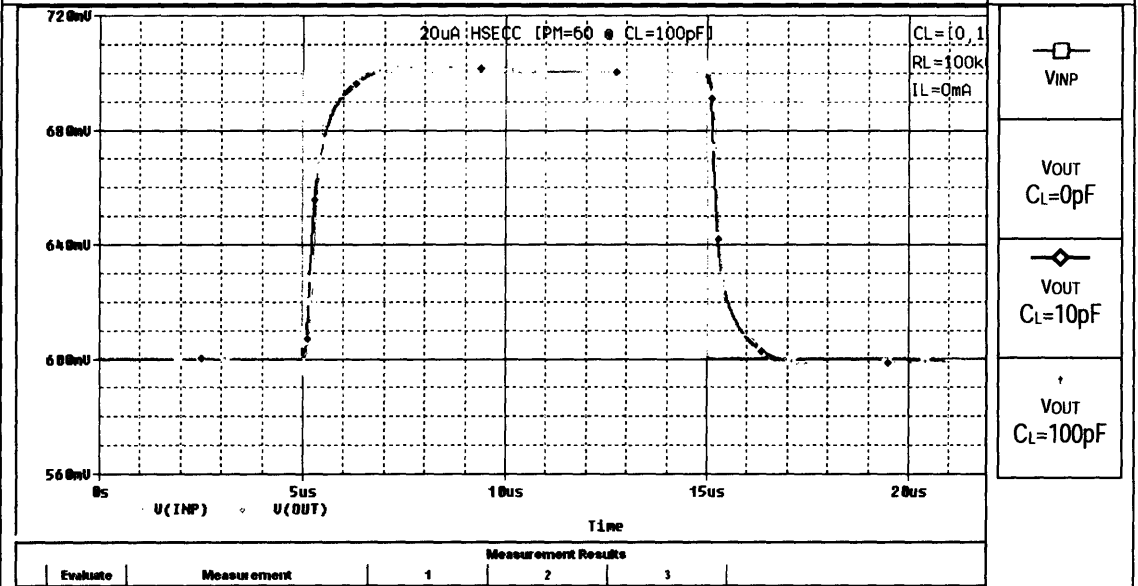
Figure C-8: Small-Signal Transient Response with C_L=0, 10, 100\text{pF} and R_L=100\text{k}\Omega
