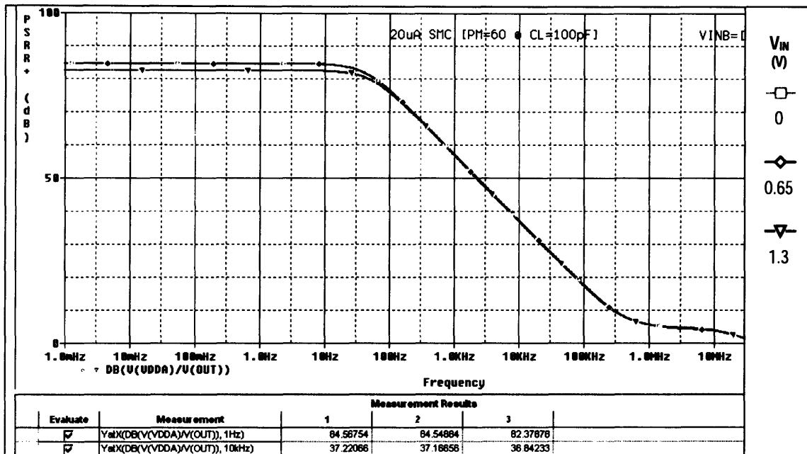
Figure A-5: PSRR+ vs Frequency with V_{IN}=0, 0.65, 1.3V
