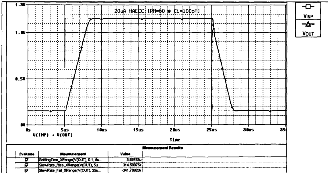
Figure D-9: Large-Signal Transient Response with C_L=100\text{pF} and R_L=100\text{k}\Omega
