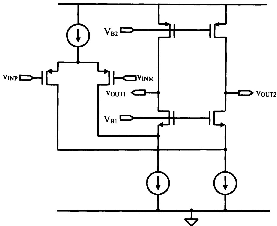
Figure 2-4: Fully Differential Folded-Cascode Input Stage [9]
