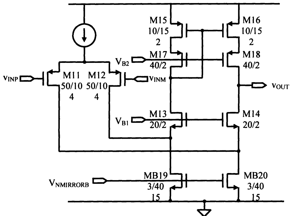
Figure 2-6: Input Stage with Transistor Sizes
