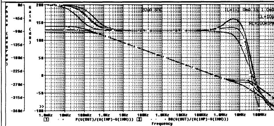
Figure A-17: Frequency Response with C_L=0\text{pF} and R_L=100\text{k}\Omega @ I_L=-1.0, -0.5, 0.0, 0.5, 1.0\text{mA}
