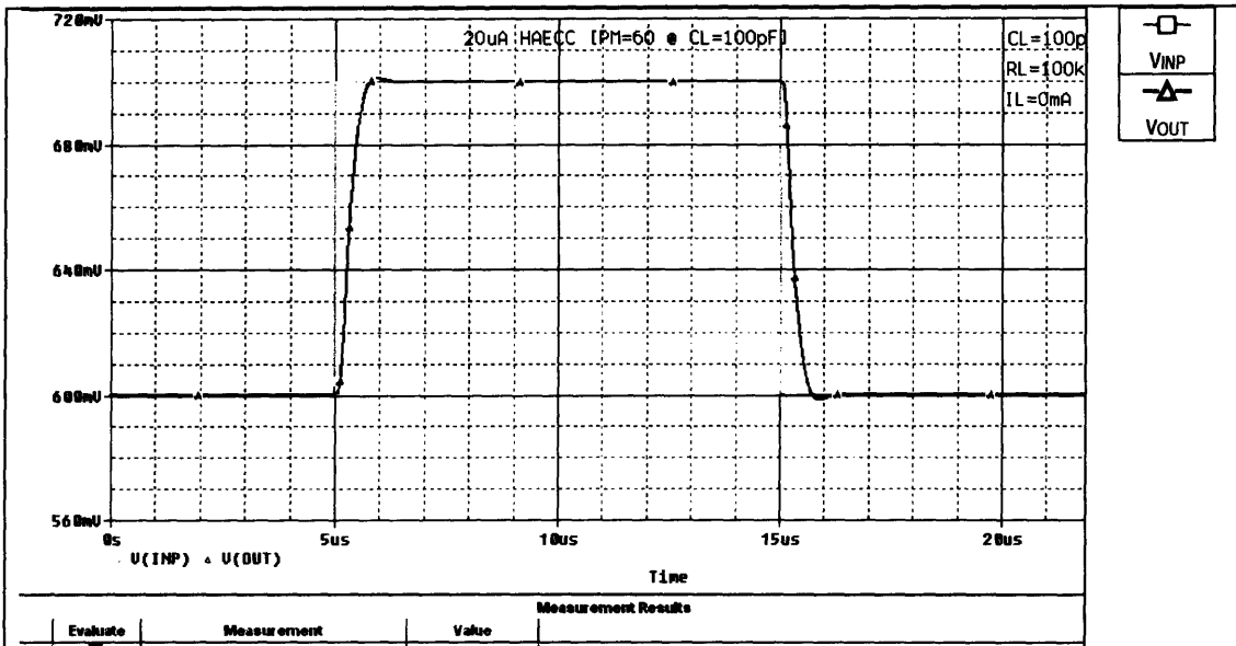
Figure D-7: Small-Signal Transient Response with C_L=100\text{pF} and R_L=100\text{k}\Omega
