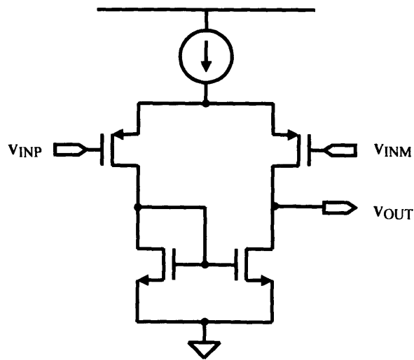
Figure 2-1: Basic Input Stage
