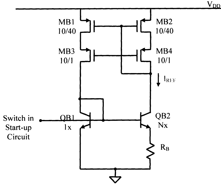
Figure 4-1: Bias Core Generating Reference Current [25], [26]
