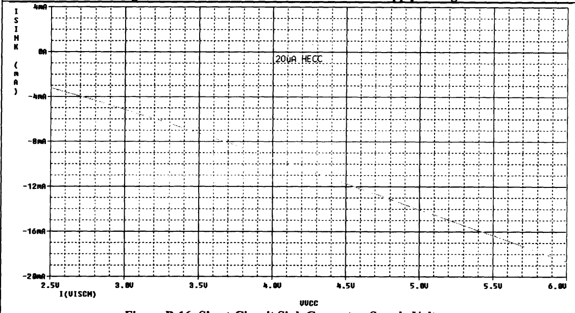
Figure B-16: Short-Circuit Sink Current vs Supply Voltage
