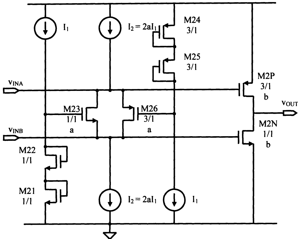
Figure 3-3: Translinear-Loop-Biased Class AB Output Stage
