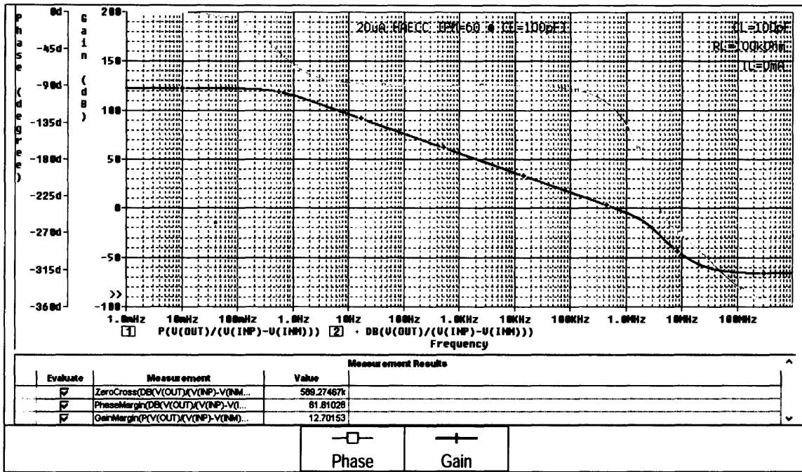
Figure 5-12: Frequency Response with C_L=100\text{pF} and R_L=100\text{k}\Omega of Proposed Micropower Op Amp with Hybrid Asymmetric Embedded Cascode Compensation (HAECC)
