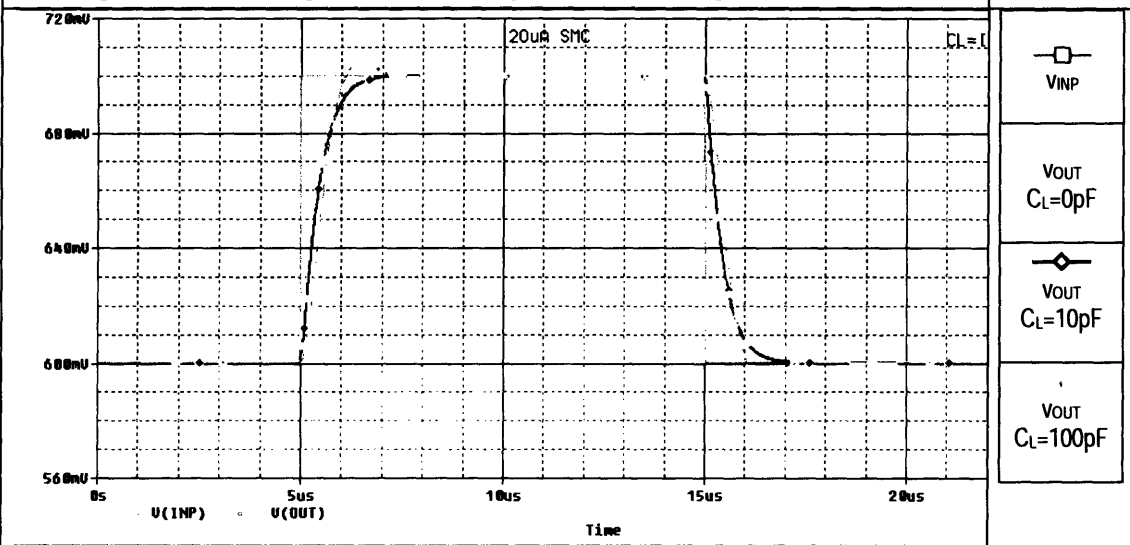
Figure A-7: Small-Signal Transient Response with C_L=100\text{pF} and R_L=100\text{k}\Omega
