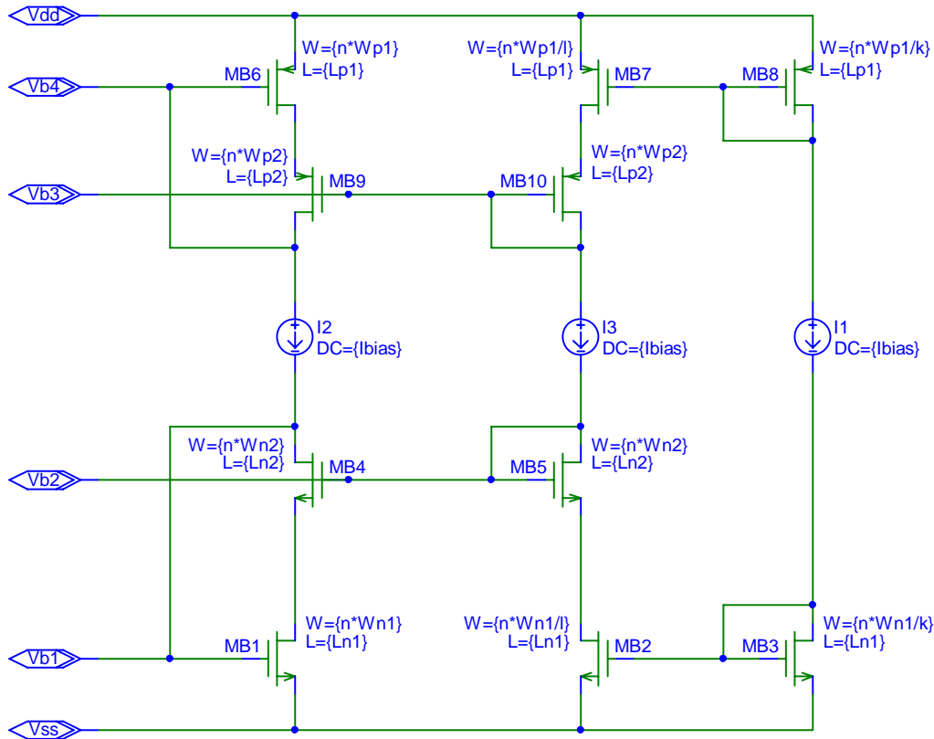
pcas_bias.sch
