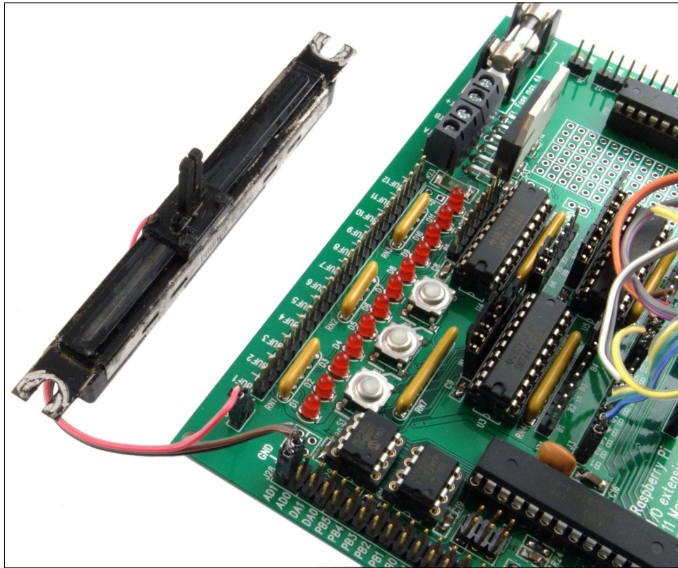
FIGURE 16-10: Connecting a potentiometer to the Gertboard's ADC pins
