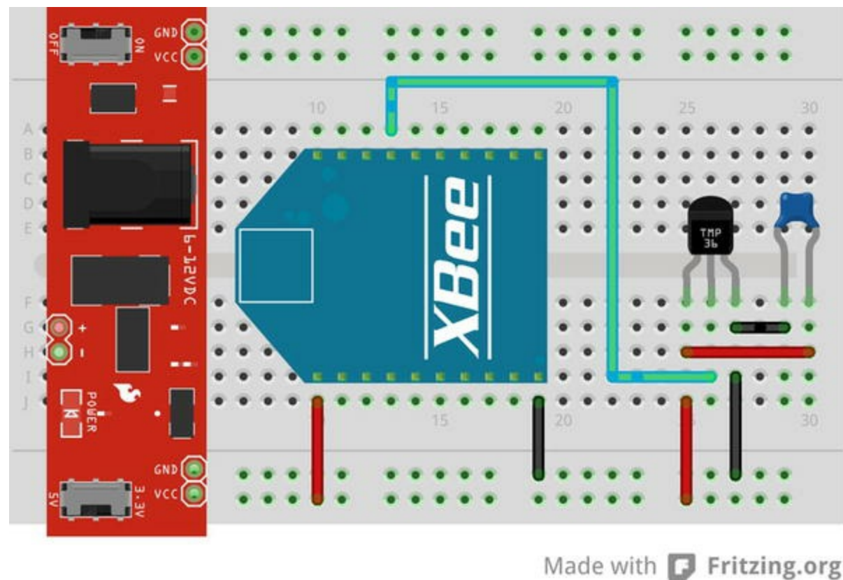
Figure 3-23. XBee temperature sensor node
