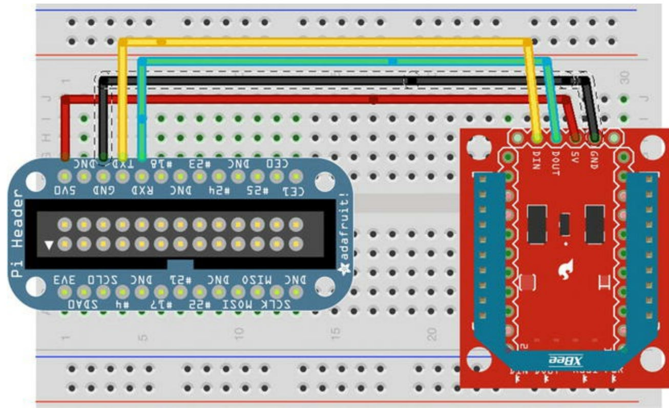
Figure 8-9. Connecting an XBee to a Raspberry Pi
