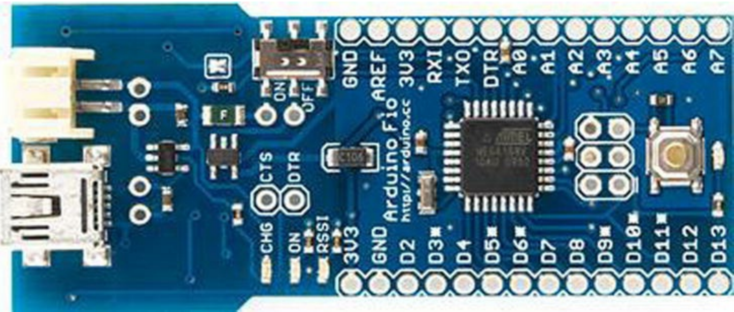
Figure 3-10. Arduino Fio (courtesy of Arduino.cc)
