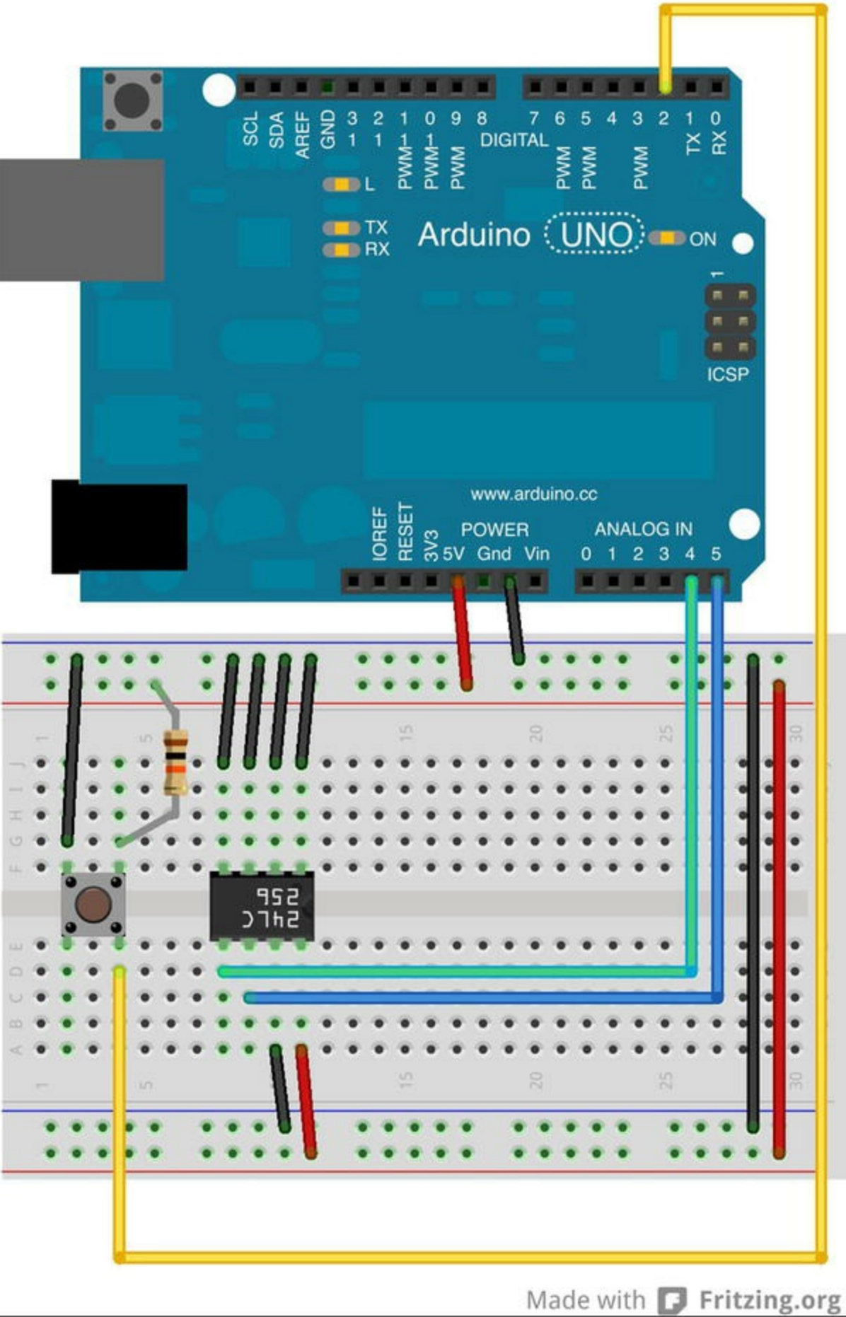
Figure 5-3. Wiring the EEPROM to the Arduino
