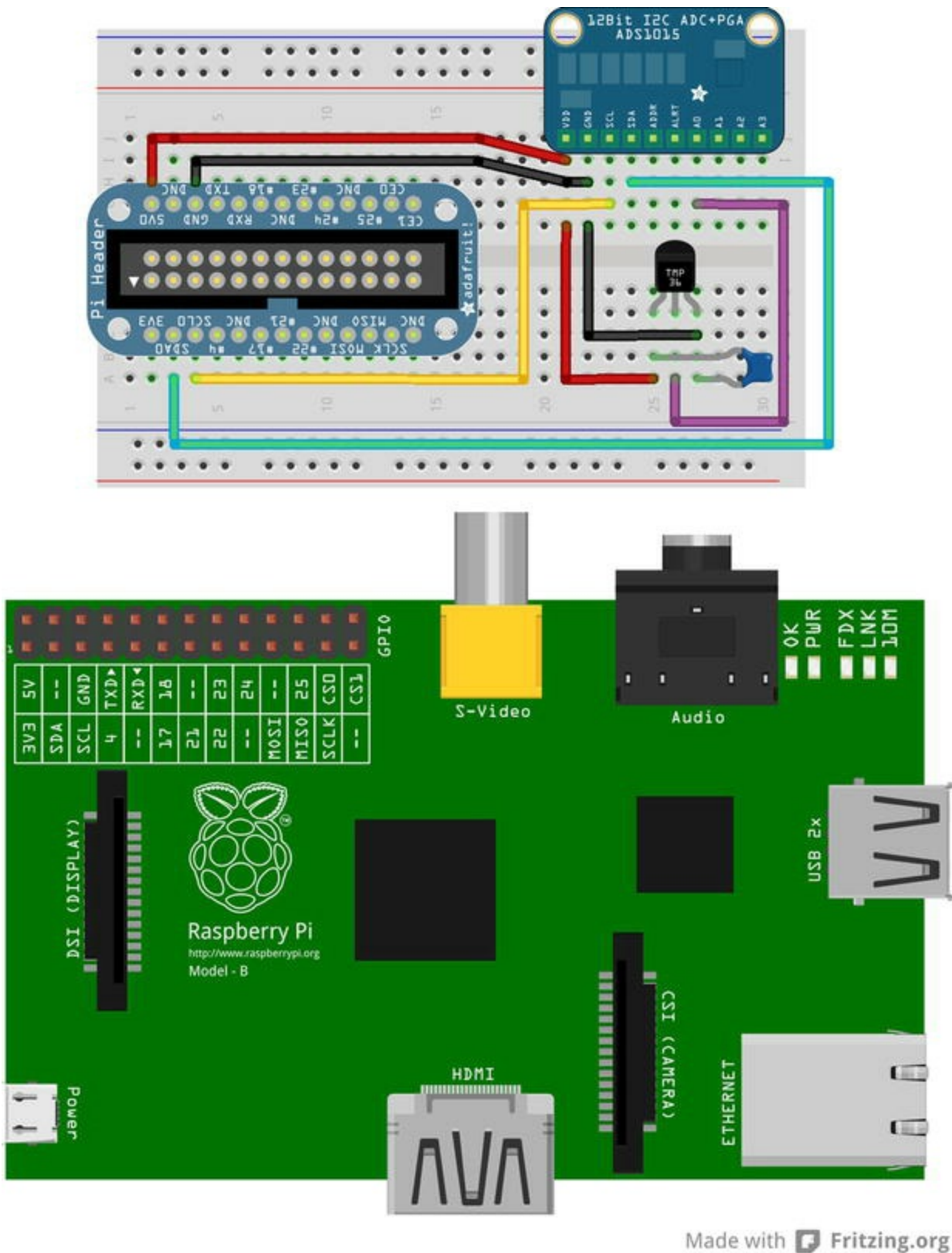
Figure 5-14. Wiring the TMP36 and ADC to the Raspberry Pi
