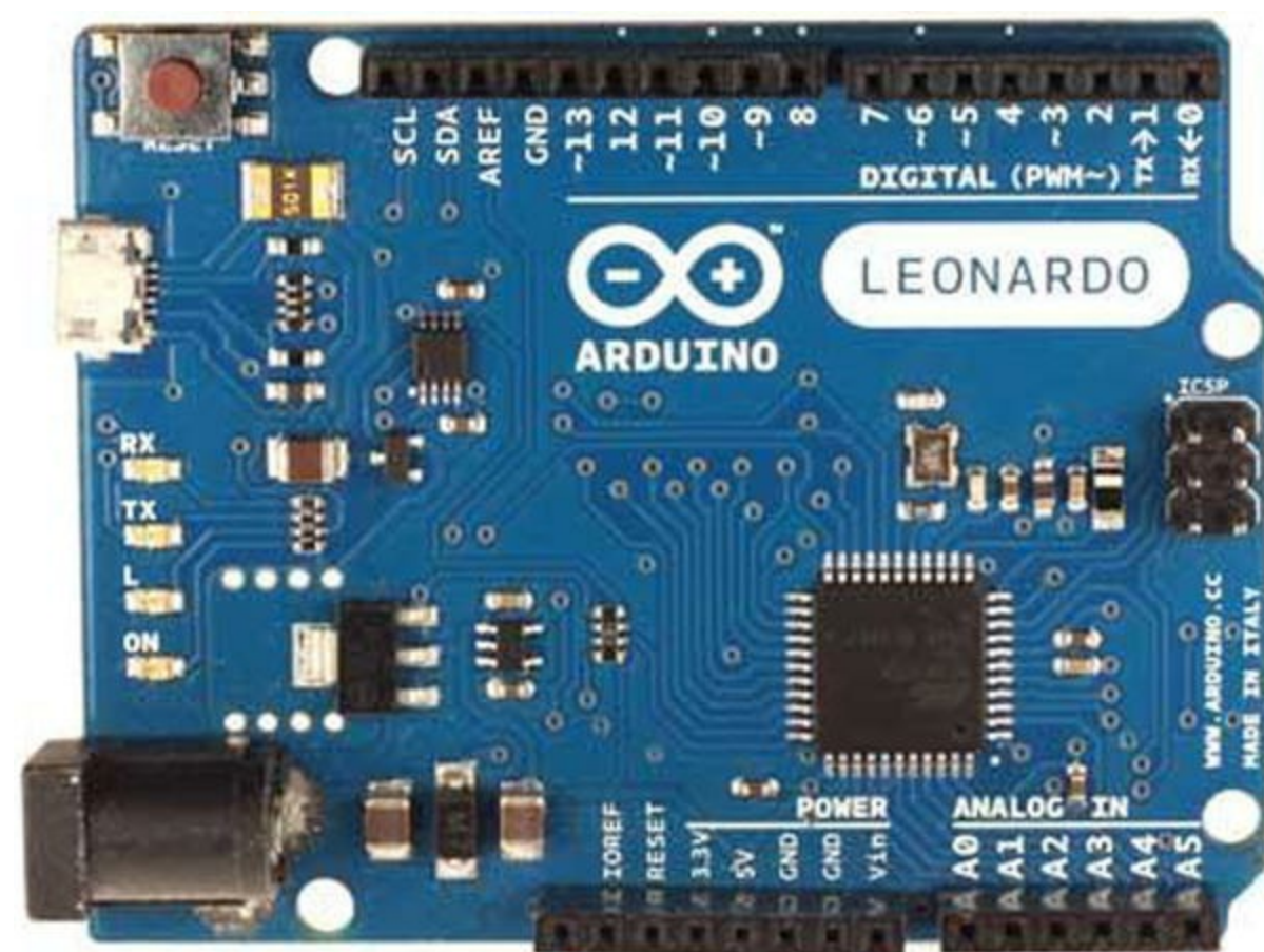
Figure 3-1. Arduino Leonardo (courtesy of Arduino.cc)
