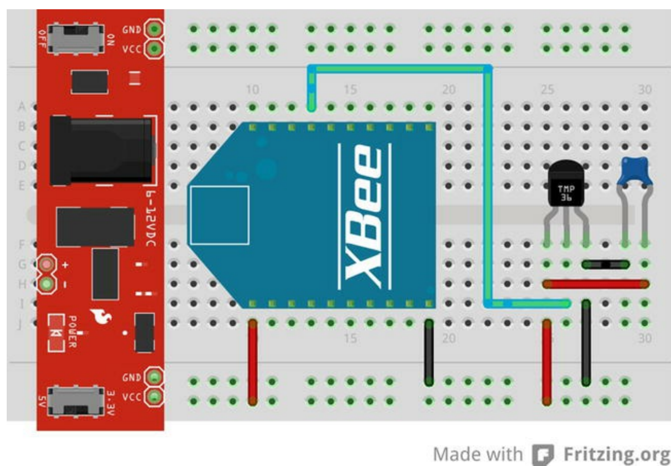
Figure 4-21. XBee sensor node
