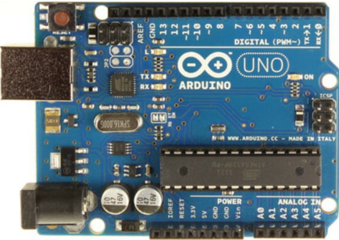
Figure 7-1. Arduino Uno (courtesy of arduino.cc)
