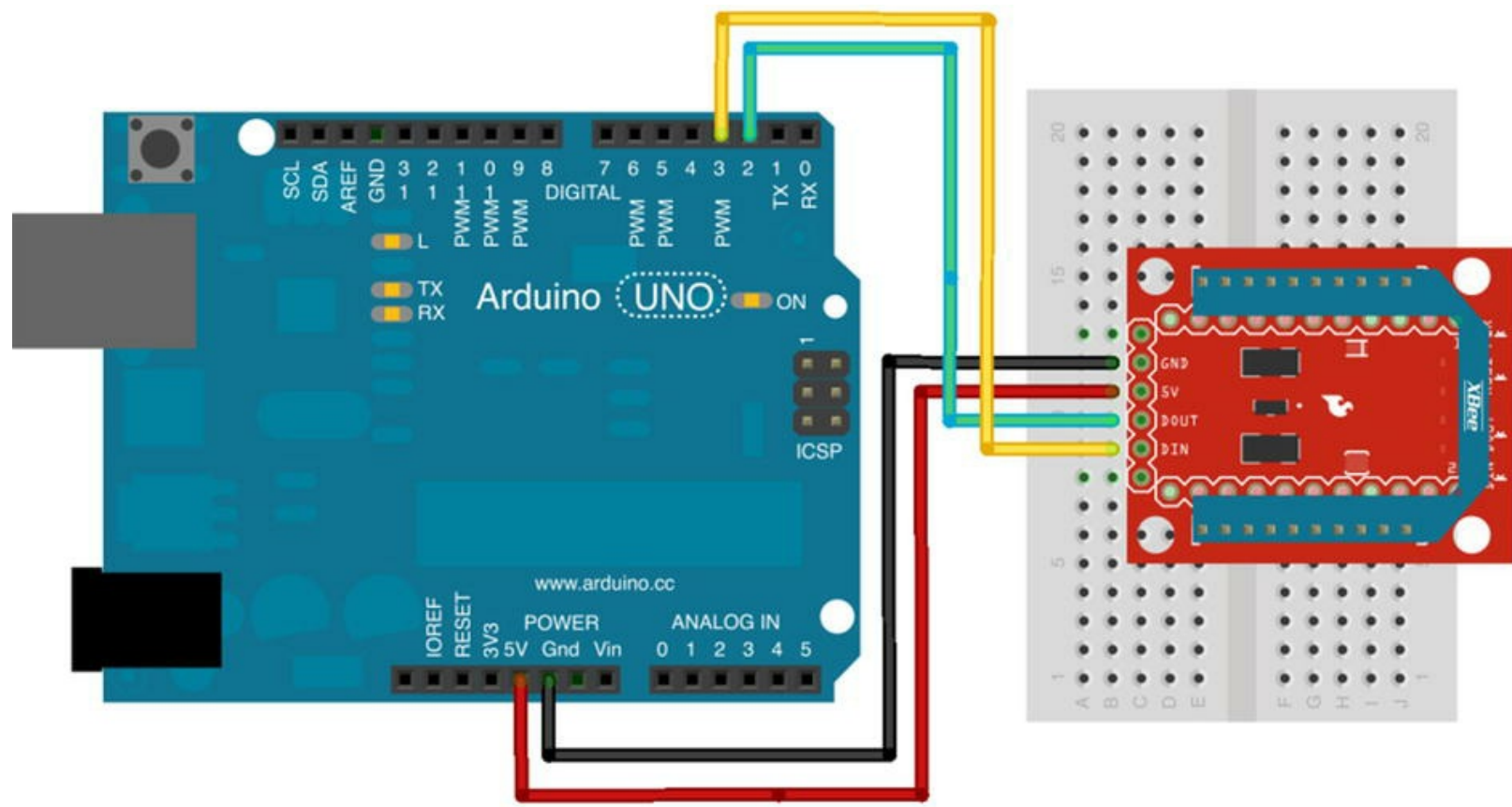
Figure 3-26. Connecting an XBee to an Arduino via a SparkFun XBee breakout board
