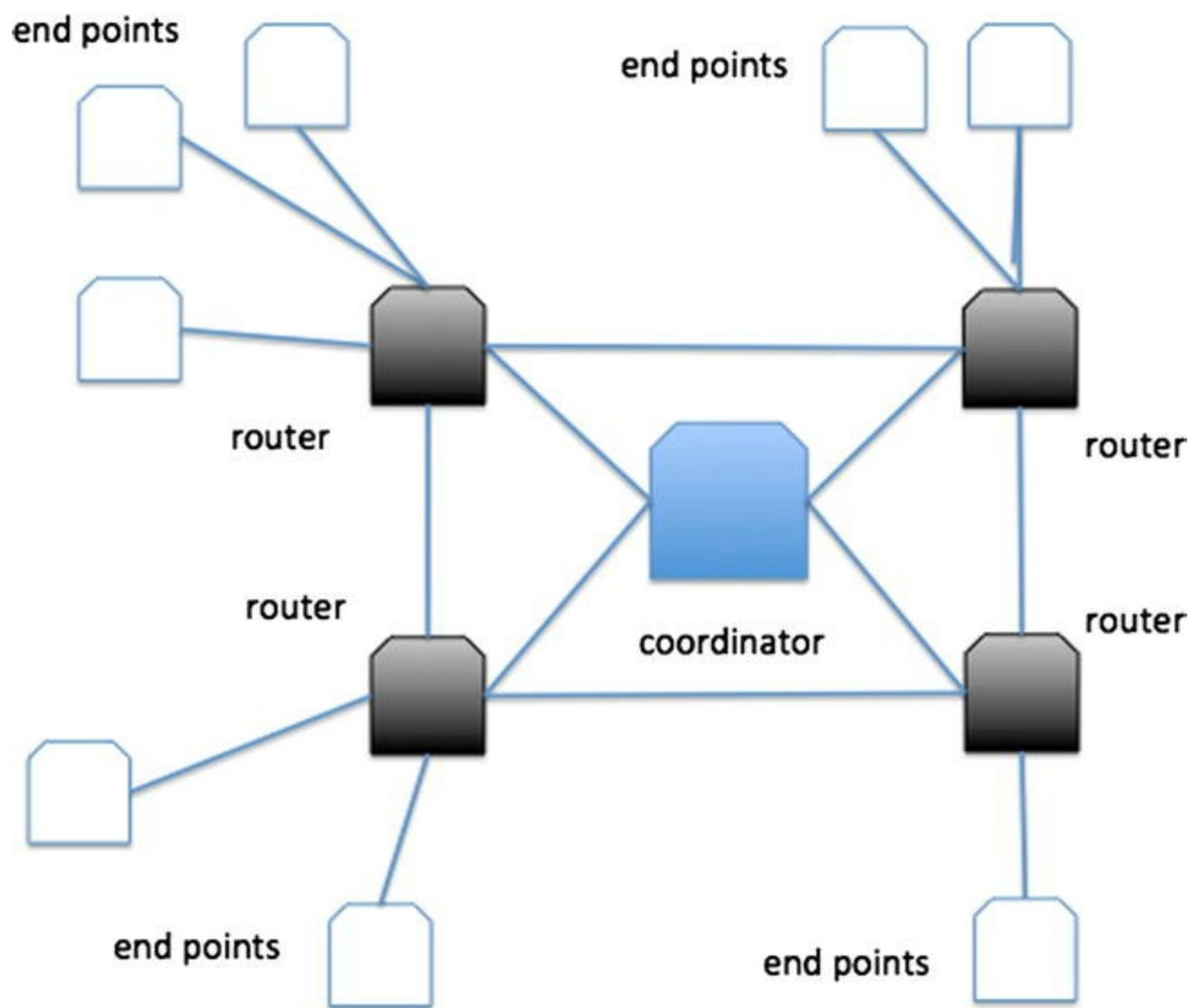
Figure 2-7. ZigBee mesh network
