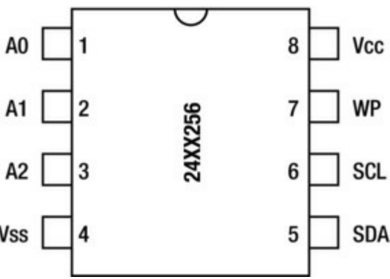
Figure 5-2. Pinout of the I2C EEPROM
