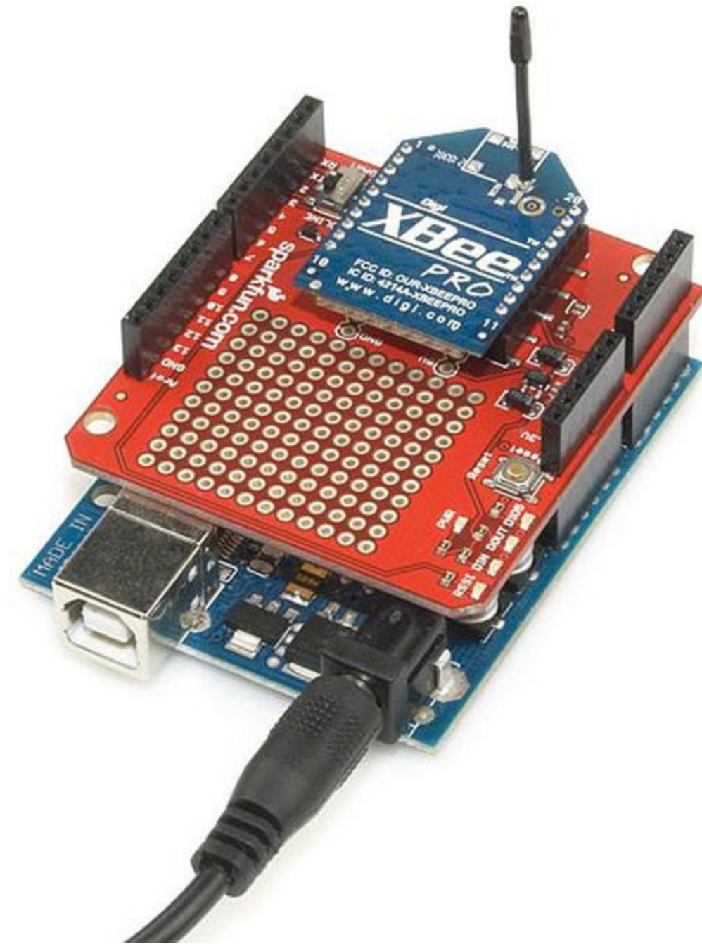
Figure 3-25. Arduino XBee shield (courtesy of SparkFun)
