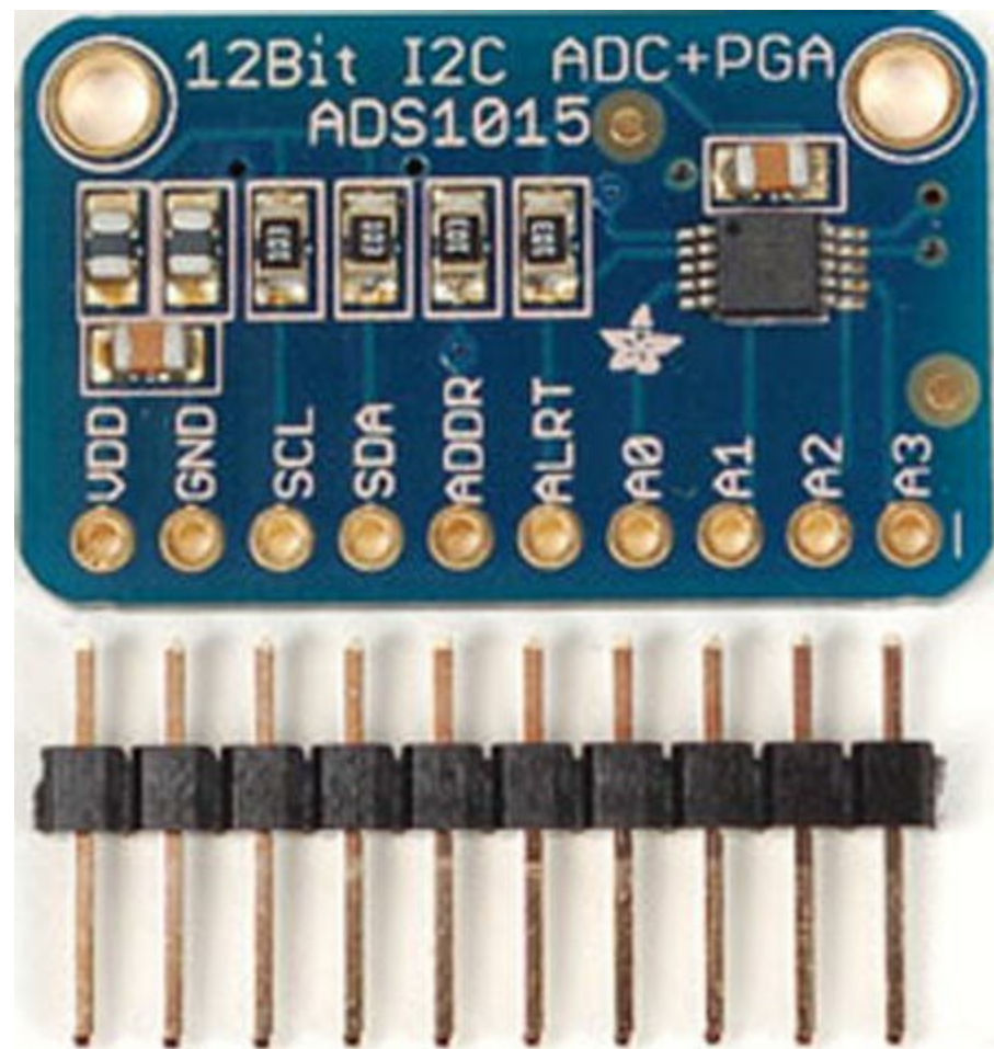
Figure 5-13. 12-Bit ADC module (courtesy of Adafruit)
