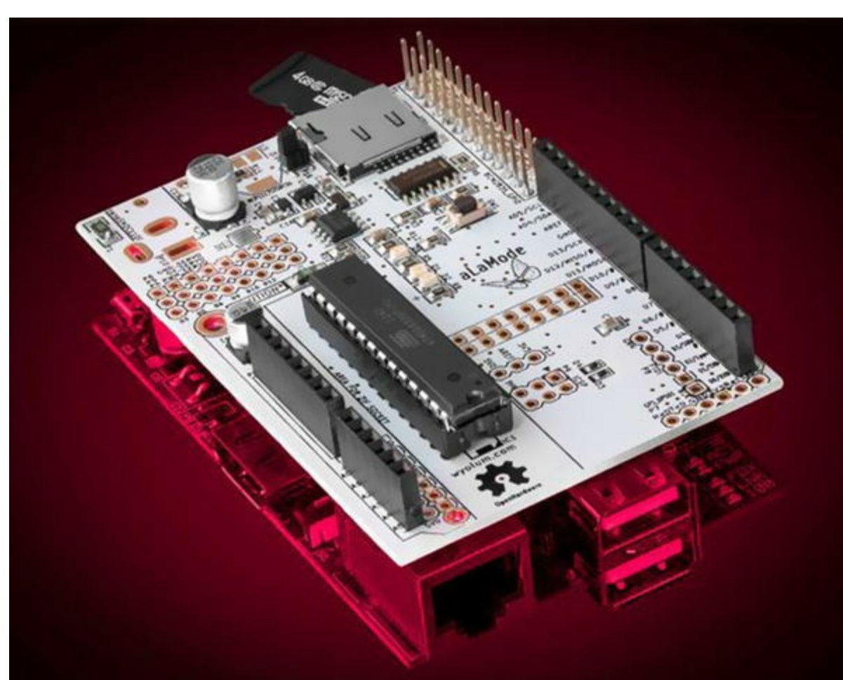
Figure 9-6. Raspberry Pi Alamode (courtesy of Seeed Studio)
