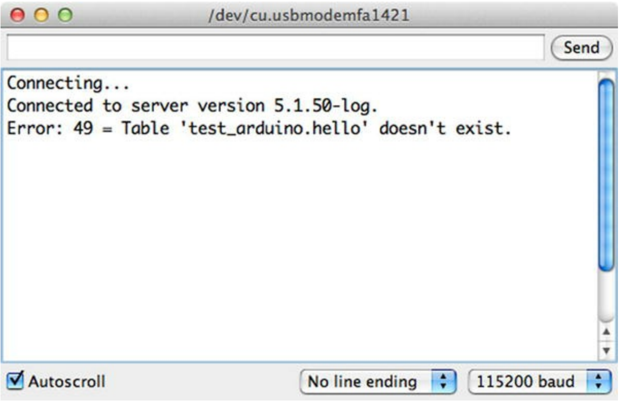
Figure 7-8. Failed query
