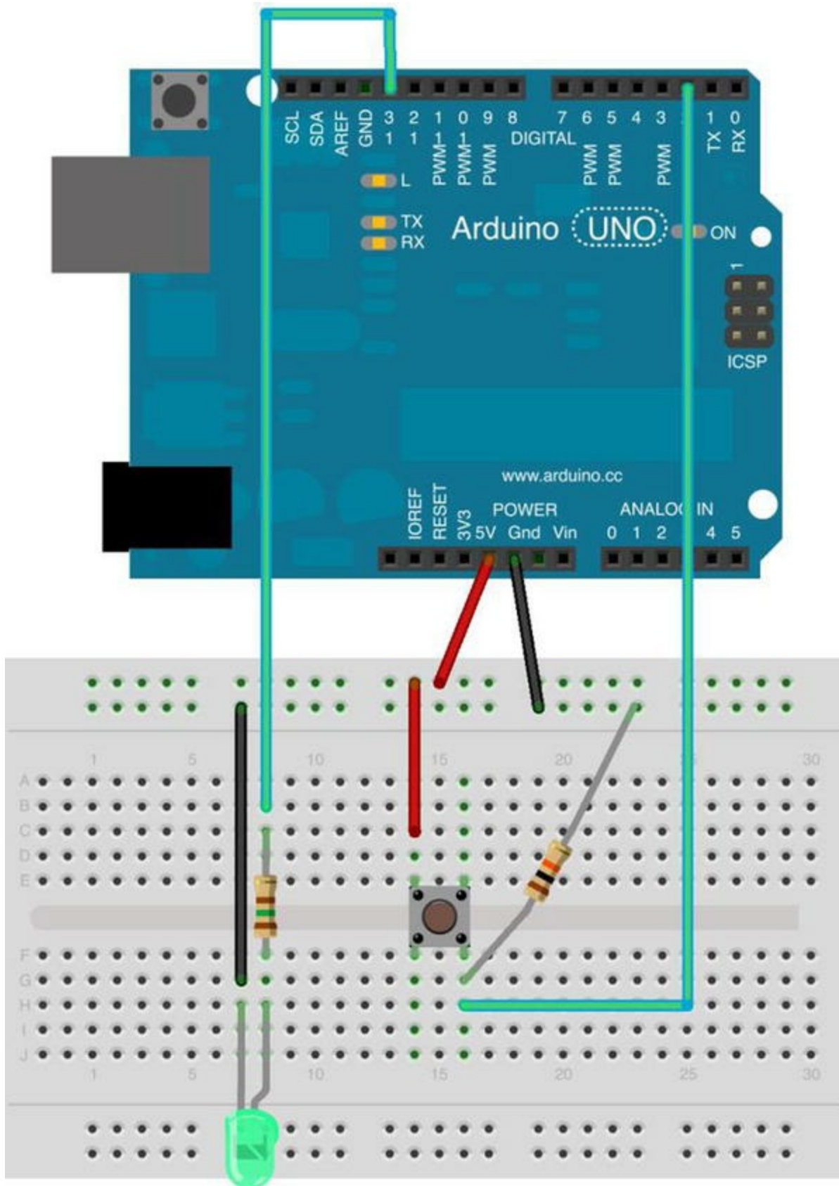
Figure 3-18. Diagram of an LED with a pushbutton
