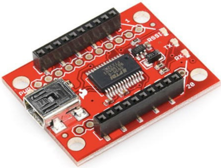
Figure 2-3. XBee Explorer USB (courtesy of SparkFun)
