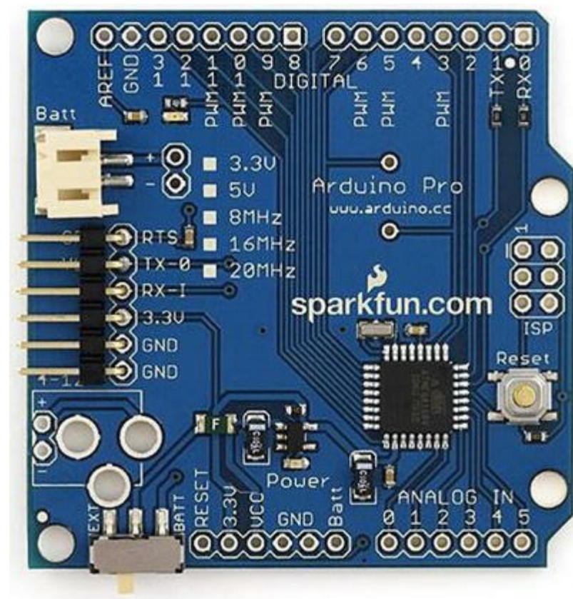
Figure 3-8. Arduino Pro (courtesy of Arduino.cc)
