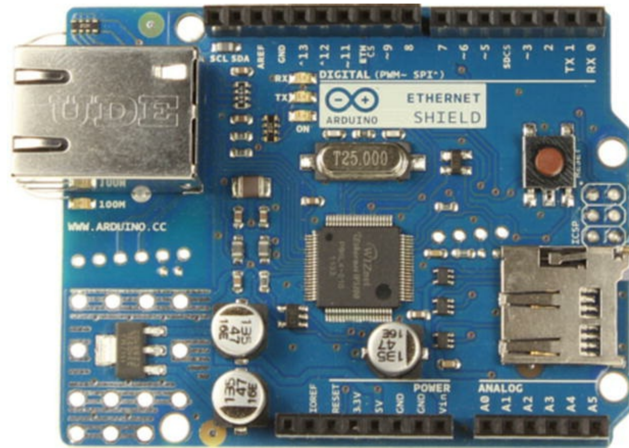
Figure 7-3. Arduino Ethernet shield (courtesy of arduino.cc)
