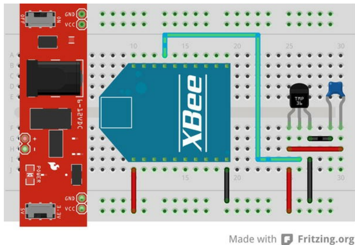
Figure 8-4. Wiring the TMP sensor node
