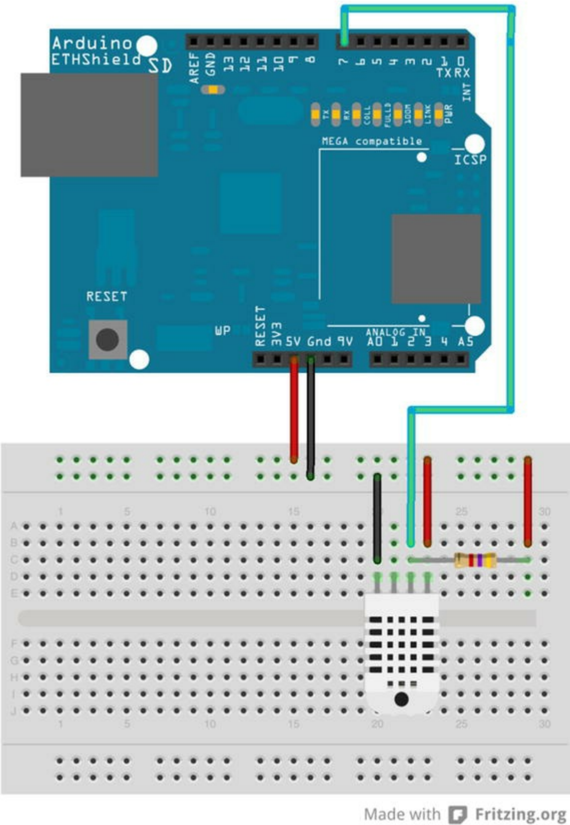
Figure 3-20. Wiring the DHT22
